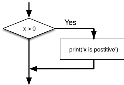
Figure 3.1: If Logic
