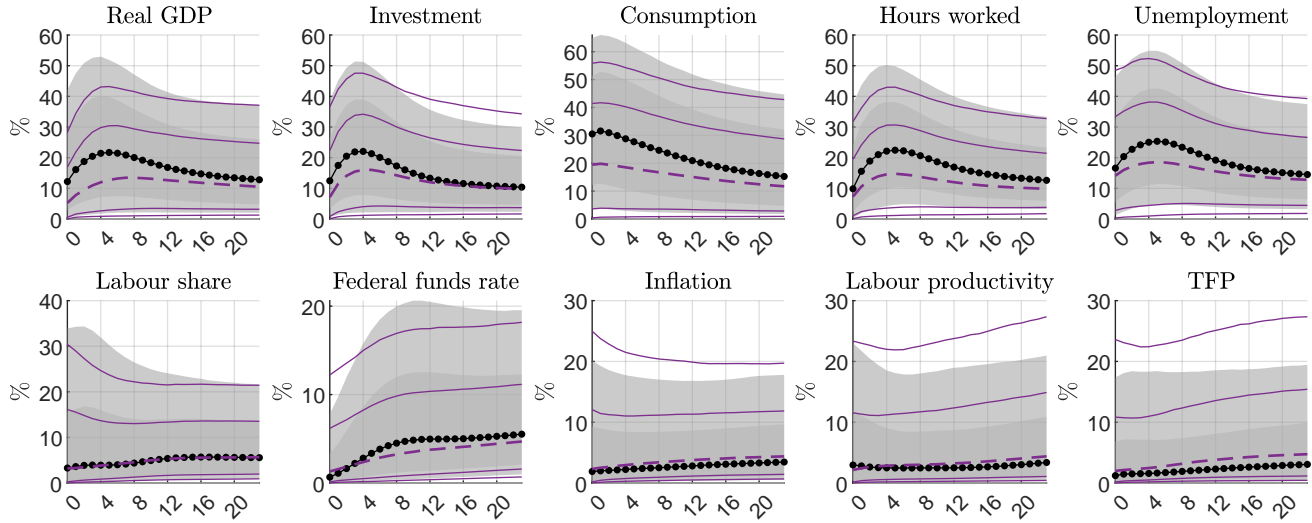
Figure H-22: Robustness for looser prior on \phi : forecast error variance decomposition
