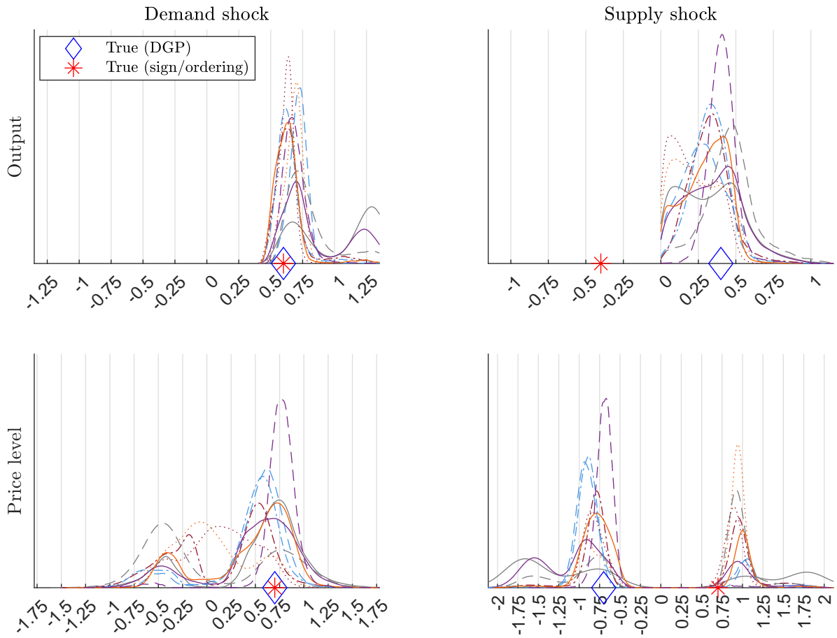
Figure G-6: Comparing normalizations: Gouriéroux et al. (2020)
