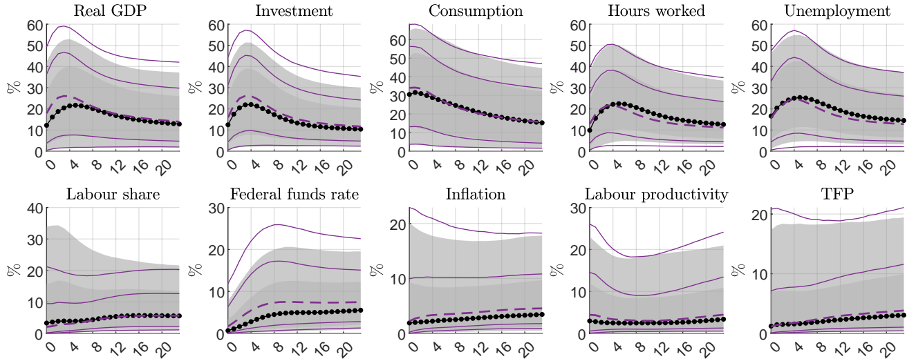
Figure H-24: Robustness for p = 4 : forecast error variance decomposition
