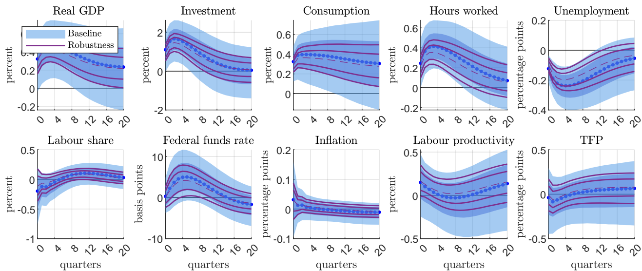
Figure H-17: Robustness for flat prior on A: impulse responses
