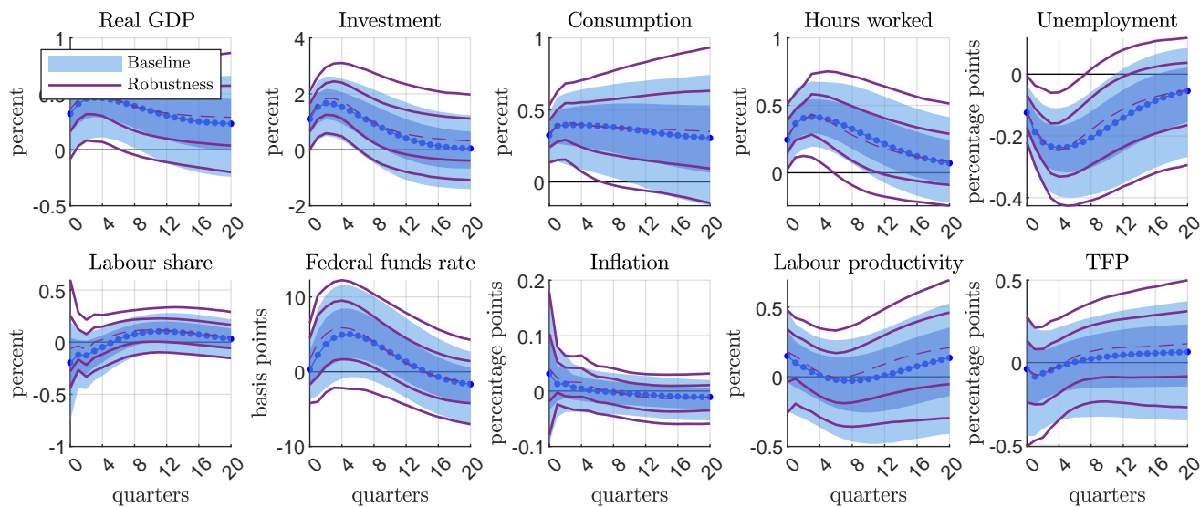
Figure H-23: Robustness for p = 4 : impulse responses
