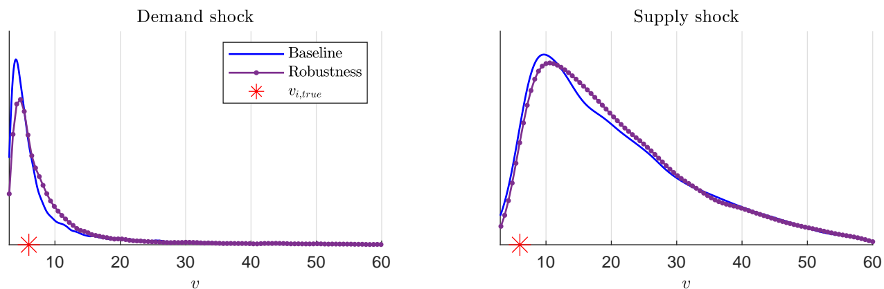
Figure G-10: Robustness for flat prior on A
