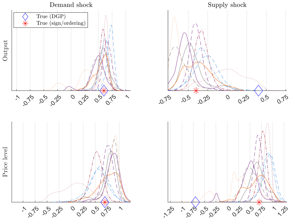
Figure G-3: Comparing normalizations: our approach
