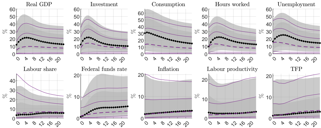
Figure H-20: Robustness for flat prior on v : forecast error variance decomposition
