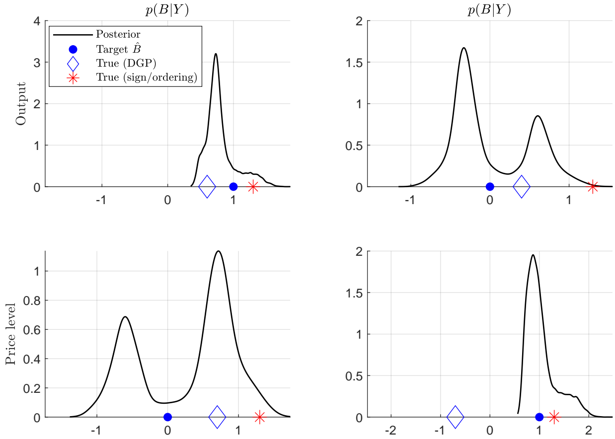
Figure G-7: Impact effect of the shocks ( B ) when the normalization targets an arbitrary matrix: \hat{B} = I_2
