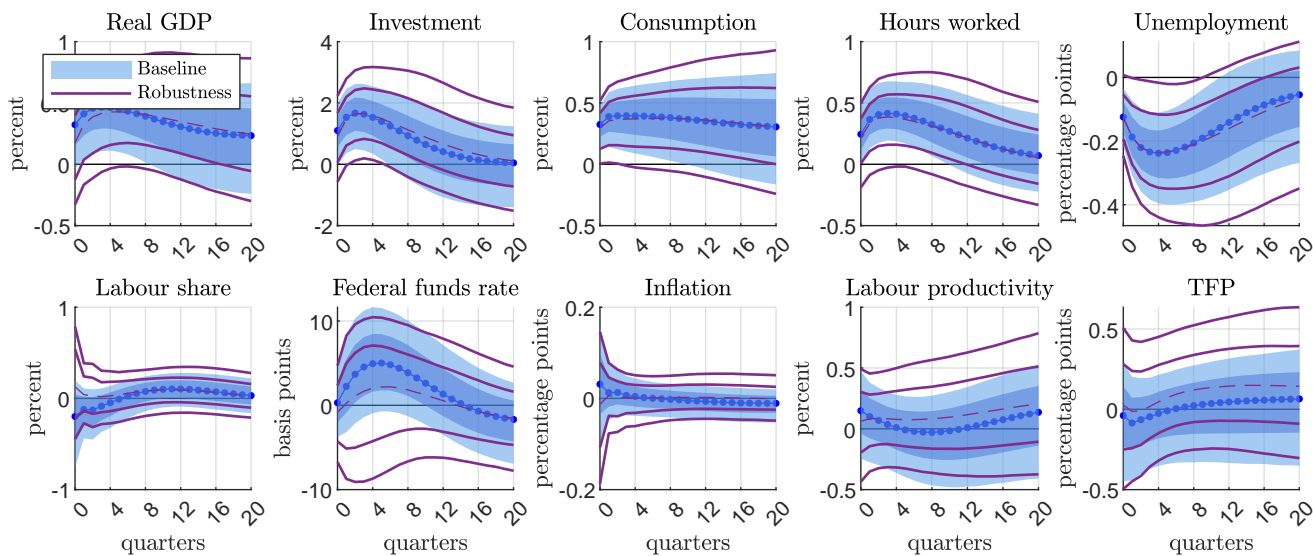
Figure H-21: Robustness for looser prior on \phi : impulse responses
