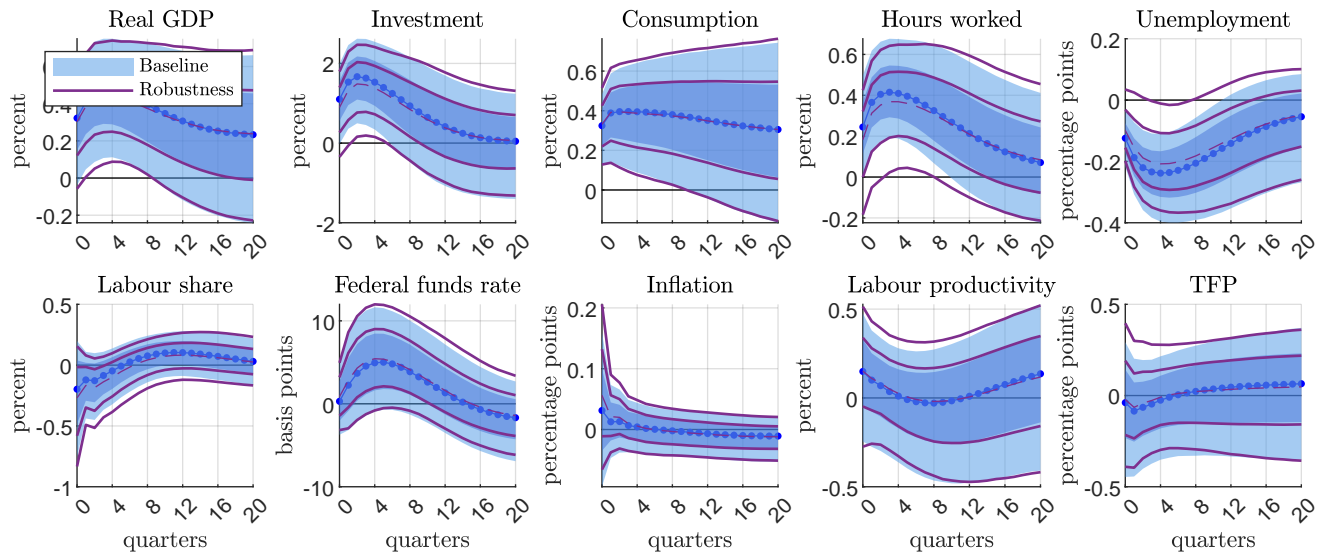
Figure H-15: Robustness computing target matrix \hat{B} in the sampler: impulse responses
