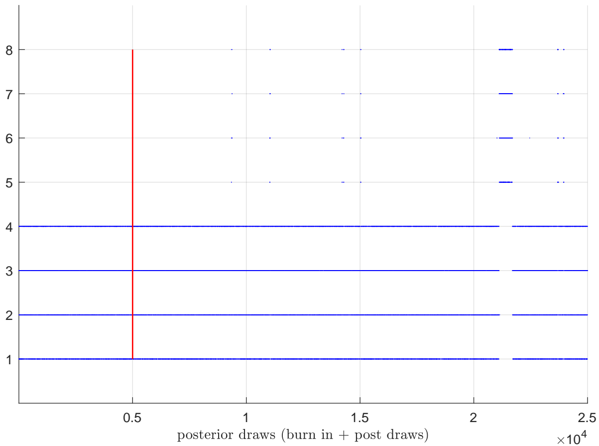
Figure G-2: Generalized LP normalization
