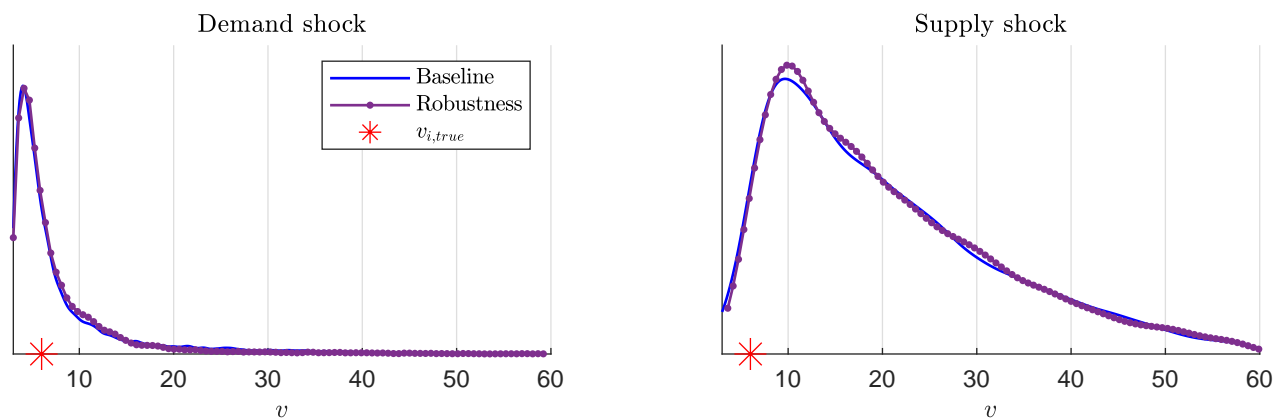
Figure G-8: Robustness when computing the target matrix in the sampler
