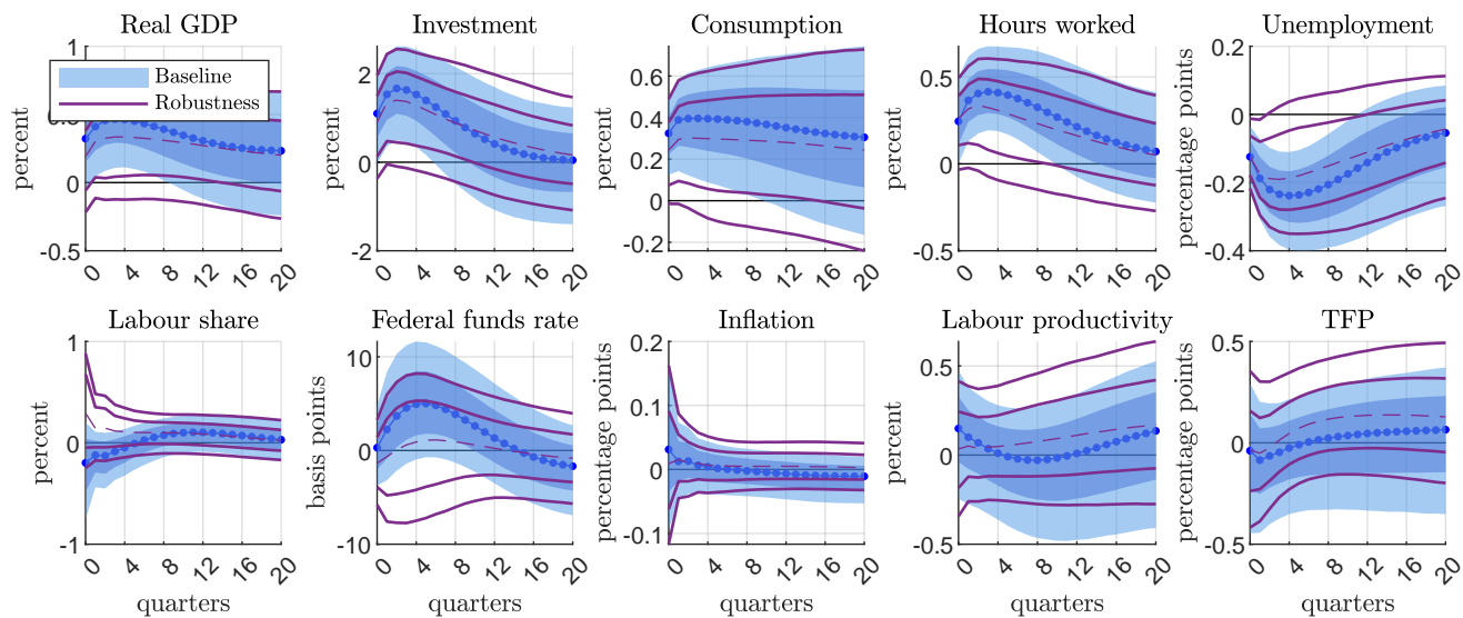
Figure H-19: Robustness for flat prior on \nu : impulse responses
