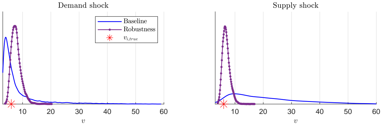
Figure G-9: Robustness for T = 1,000
