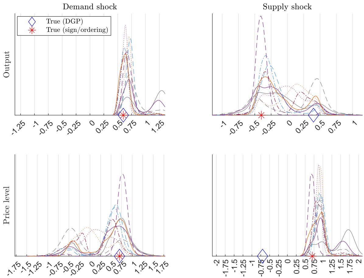
Figure G-5: Comparing normalizations: Lanne et al. (2017)
