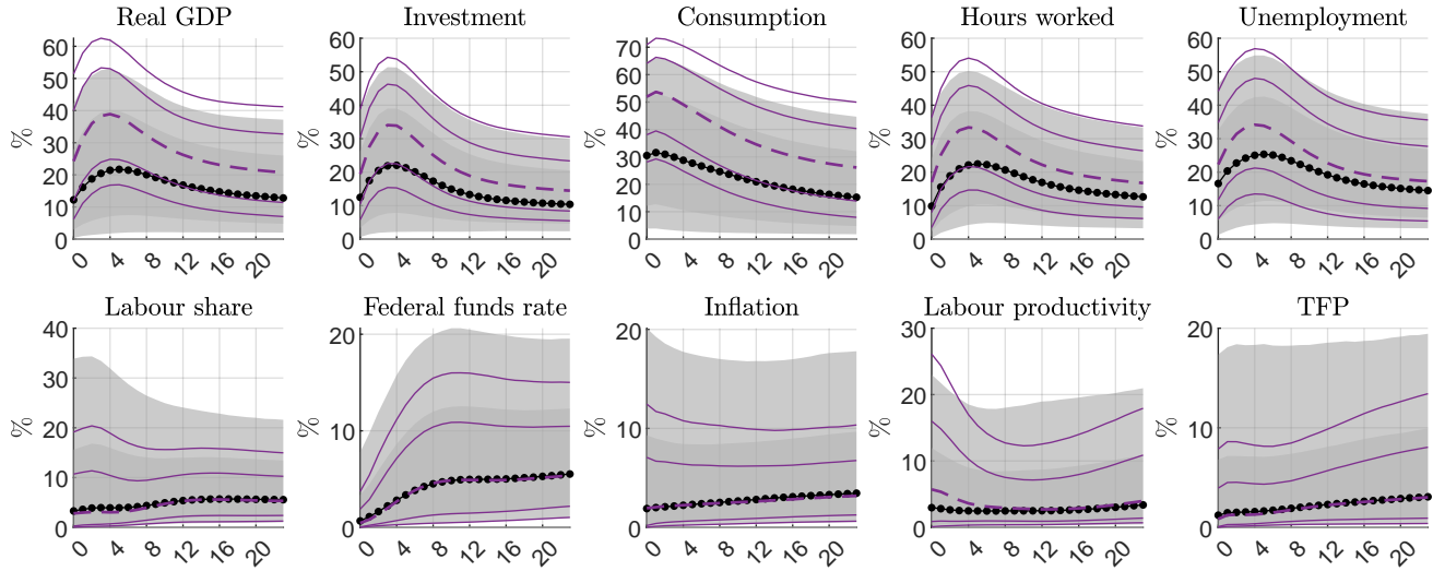
Figure H-18: Robustness for flat prior on A : forecast error variance decomposition
