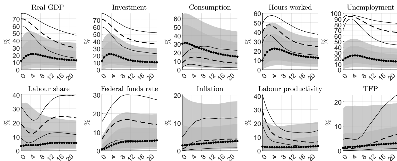
Figure H-14: Forecast error variance decomposition Shock 3: demand shock
