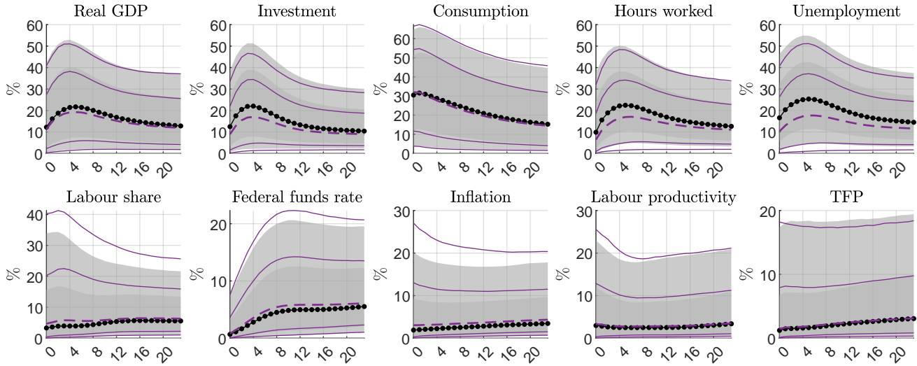
Figure H-16: Robustness computing target matrix \hat{B} in the sampler: forecast error variance decomposition
