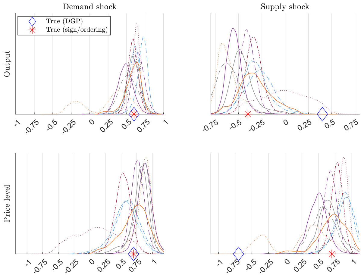
Figure G-4: Comparing normalizations: Jarociński (2024)
