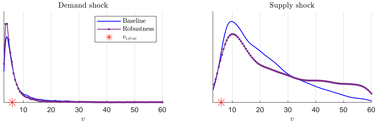
Figure G-11: Robustness for flat prior on v
