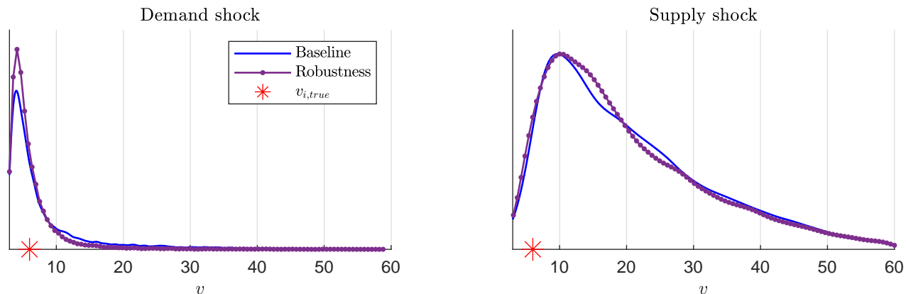
Figure G-12: Robustness for looser prior on \phi ( \lambda_1 = 0.2 rather than 0.1 using the notation in Canova, 2007)
