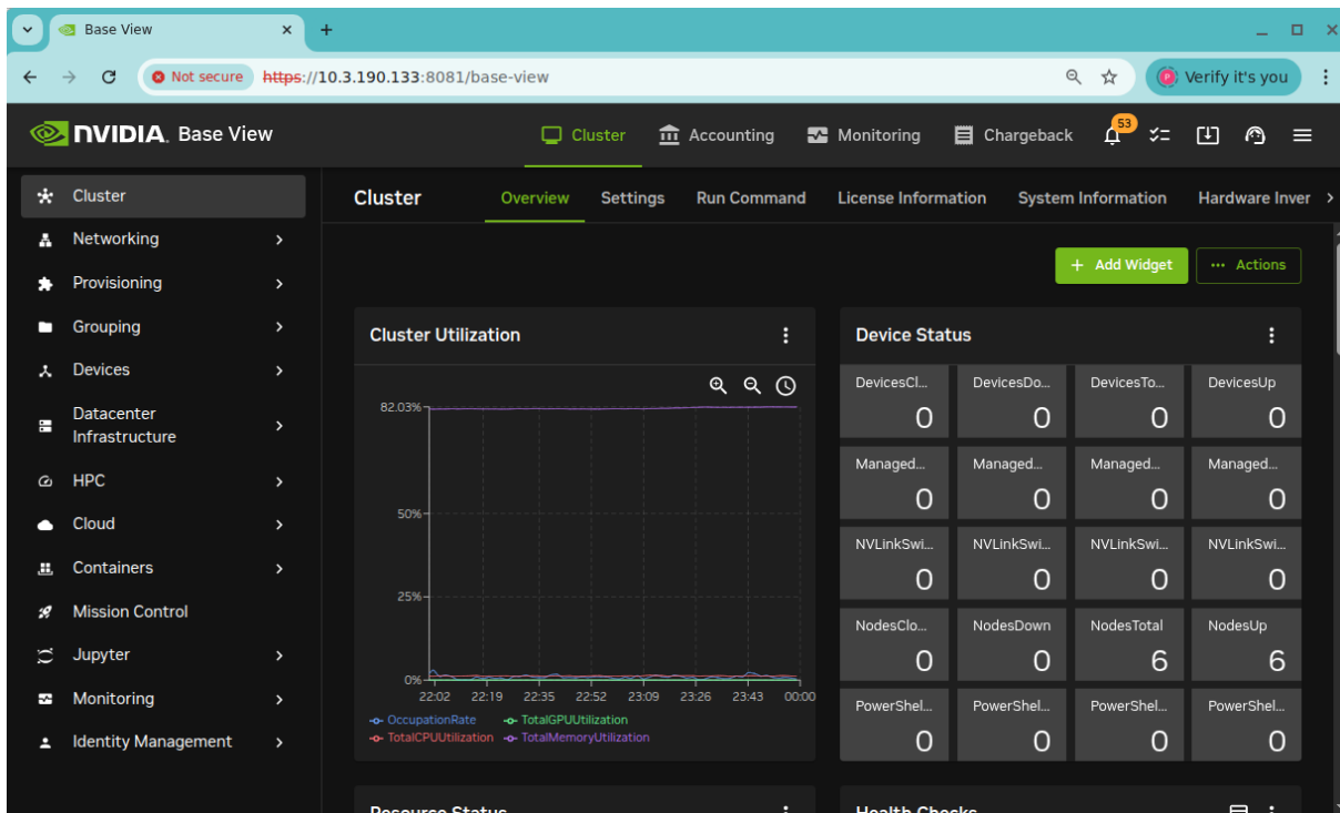
Figure 2.3: Cluster Overview
