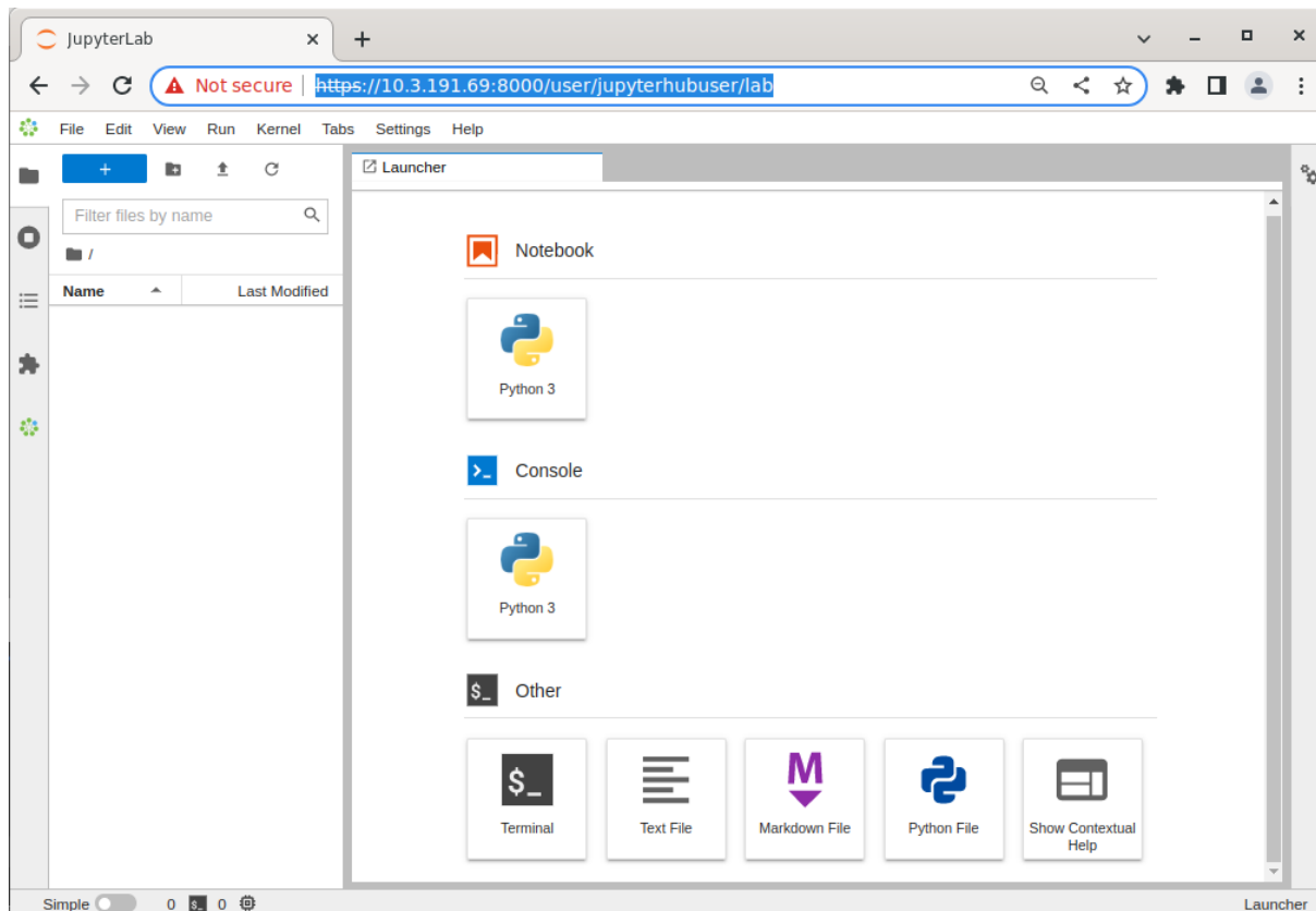
Figure 16.4: JupyterLab Launcher
