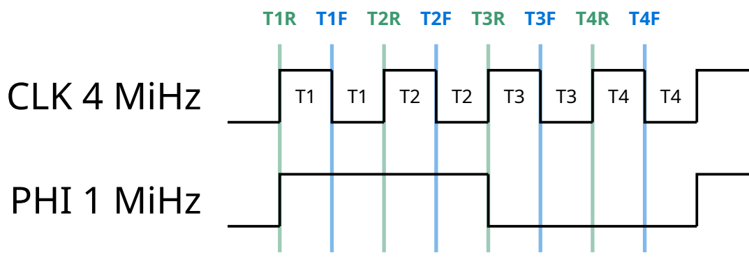
Figure 2.2: Clock edges in a machine cycle
