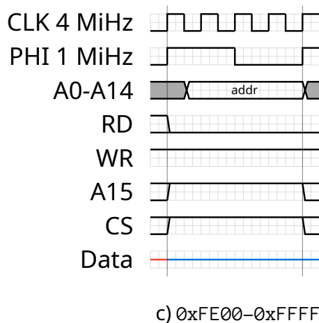
Figure C.8: External bus CPU read machine cycles
