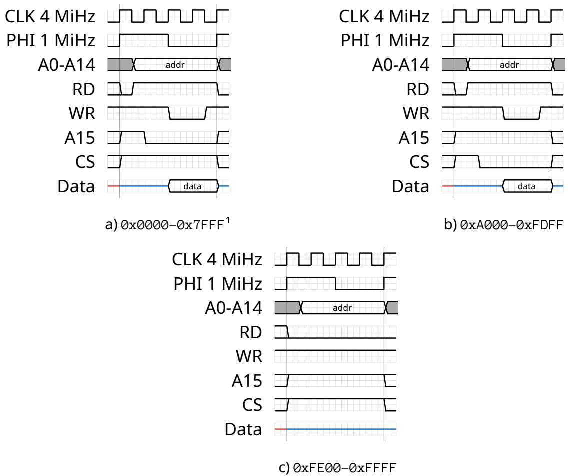
Figure C.9: External bus CPU write machine cycles
