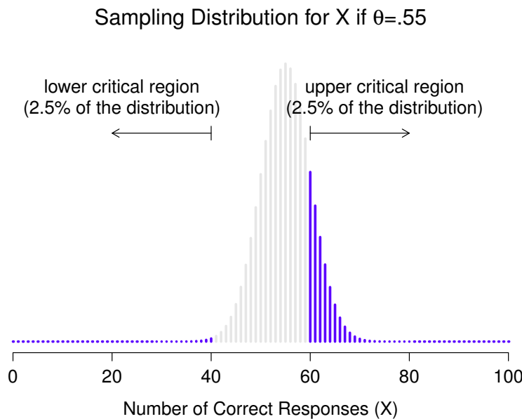
Figure 8.5: Sampling distribution under the alternative hypothesis for a population parameter value of \theta = 0.55 . A reasonable proportion of the distribution lies in the rejection region.
