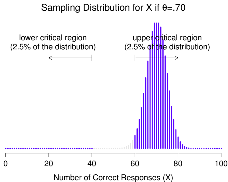
Figure 8.6: Sampling distribution under the alternative hypothesis for a population parameter value of \theta = 0.70 . Almost all of the distribution lies in the rejection region.
