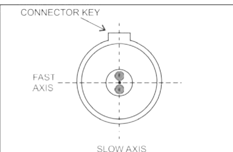
Figure 5: PM Axis Alignment aligned to the slow axis
