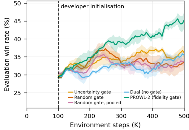
Figure 6: Gate controls on Terran 5v5. All arms branch from the same checkpoint at 100K steps, where the developer is initialised (dashed line). Dual has no gate; the other arms differ only in which states the gate quarantines. Mean over three seeds with \pm 1 s.e. bands.
