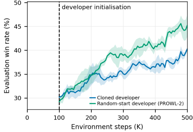
Figure 7: Developer initialisation on Terran 5v5. PROWL-2 with a randomly initialised developer, as in the reported runs, against a developer cloned from the task actor at the branch point. Mean over 3 seeds with \pm 1 s.e. bands.
