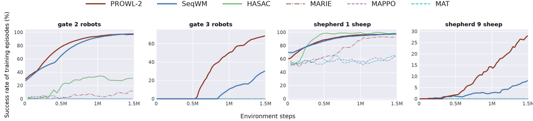
Figure 4: Learning curves on MQE. Success rate of training episodes over 1.5M environment steps on Gate-2, Gate-3, Shepherd-Easy, and Shepherd-Hard; mean over three seeds.
