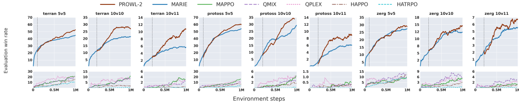
Figure 2: Learning across nine SMACv2 combat scenarios. Panels run left to right through Terran , Protoss and Zerg , each at 5v5, 10v10 and 10v11 combat. Curves report the mean evaluation win rate across three seeds. Upper panels: PROWL-2 versus its MARIE backbone; lower panels: model-free baselines. Vertical dashed lines mark the branch point, where the developer is initialised (Section 5.1).
