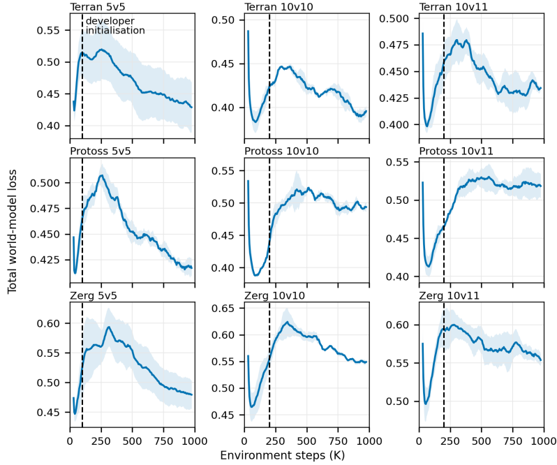
Figure 8: Total world-model loss of MARIE on SMACv2. Mean over seeds with \pm 1 s.e. bands. Dashed lines mark the developer initialisation points. All arms are identical before the branch, so only MARIE is shown.
