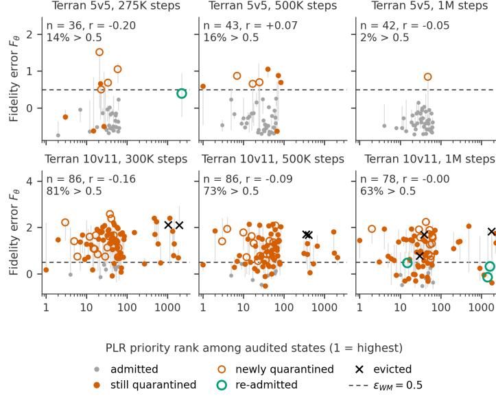
Figure 5: Audited start states at one gate tick , at three points in training (Terran 5v5 and Terran 10v11, seed 1 of the reported runs; F_\theta recomputed offline from the checkpoint at each step). Horizontal axis: priority rank in \mathcal{B}_G (1 = highest, log scale); vertical axis: fidelity error F_\theta (Eq. 6); dashed line: \epsilon_{WM} = 0.5 . Markers give the verdict at that tick: admitted, newly quarantined, still quarantined (quarantined earlier, whether it passed or failed this audit), re-admitted after a second consecutive pass, or evicted after a sixth failure. n is the number of audited states, which can fall below 64 because states with fewer than 8 recorded steps left are not audited; “> 0.5” is the share of audited states, new and re-audited, above \epsilon_{WM} .
