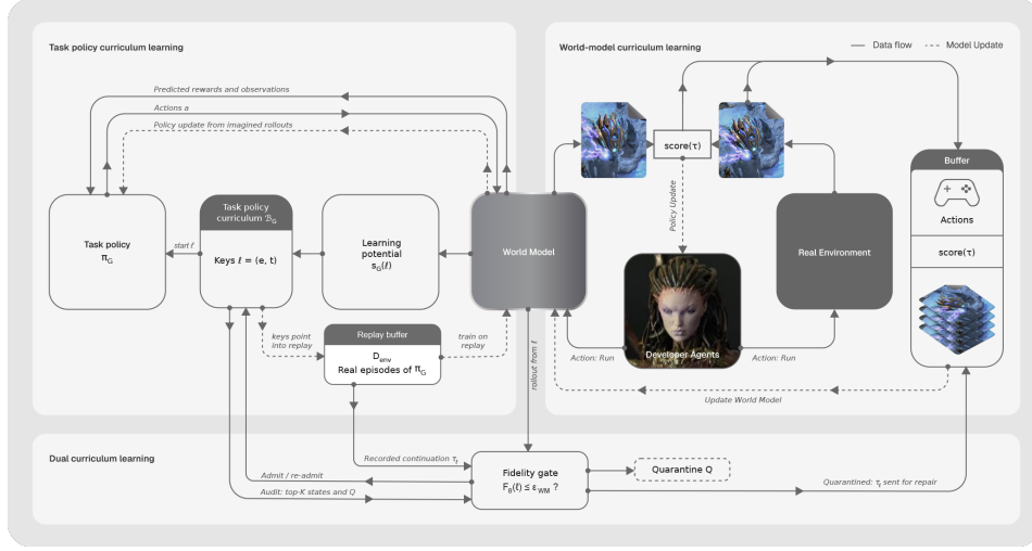
Figure 1: Overview of PROWL-2 , with the three parts described in Section 4: task policy curriculum learning (top left), world-model curriculum learning (top right) and dual curriculum learning (bottom).
