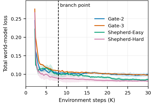
Figure 10: Total world-model loss of SeqWM on MQE over the first 30K environment steps, mean over three seeds with \pm 1 s.e. bands. Curves start after the 2K-step random warm-up. The dashed line marks the branch point.
