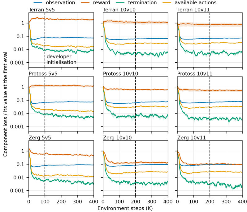
Figure 9: World-model loss terms of MARIE on SMACv2, each divided by its value at the first evaluation (log scale); mean over seeds with \pm 1 s.e. bands. Dashed lines mark the developer initialisation points.
