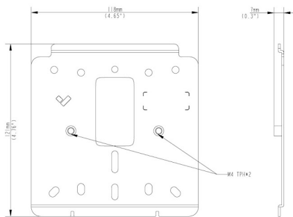
Metal mount plate
