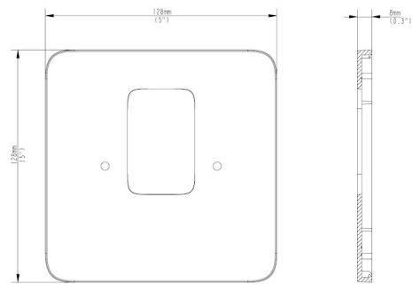
Plastic cover
