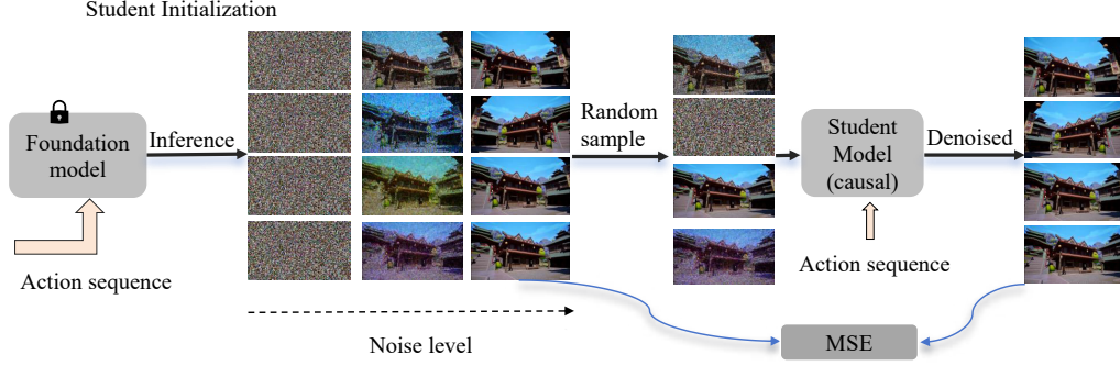
Figure 9: Causal Student Model Initialization via ODE Trajectories. The proposed initialization method stabilizes subsequent distillation training by deriving a few-step causal student model from the bidirectional teacher model through optimal ODE trajectory sampling.
