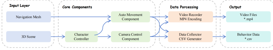
Figure 3: Overview of Our Data Production Pipeline based on Unreal Engine.
