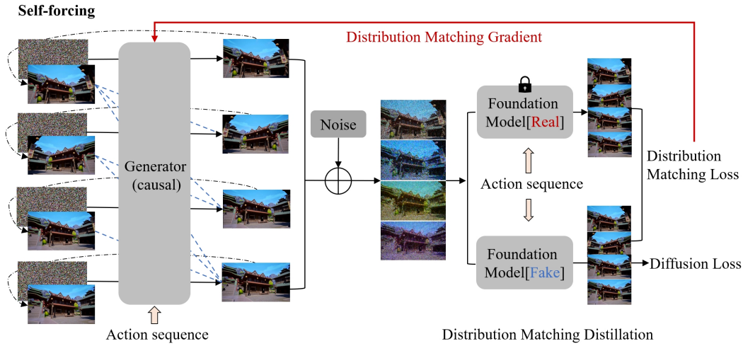
Figure 10: Overview of Causal Diffusion Model Training via Self-Forcing. The distillation process aligns the student model’s distributions with the teacher model’s through self-conditioned generation. This approach effectively mitigates error accumulation while maintaining the generation quality.
