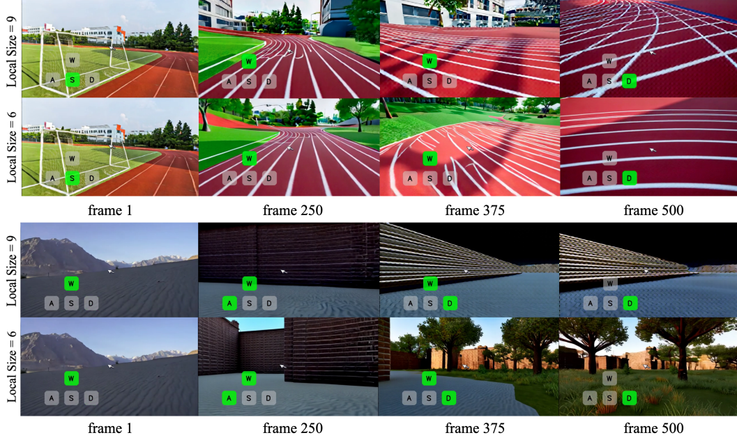
Figure 16: Qualitative Comparison on Different Local Size for KV-cache. Larger local size cause artifacts in long sequences while smaller local size can keep a balance between visual quality and content fidelity.
