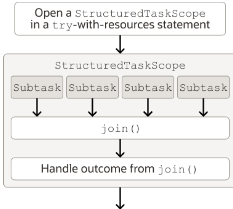
Figure 14-2 Using the StructuredTaskScope Class
