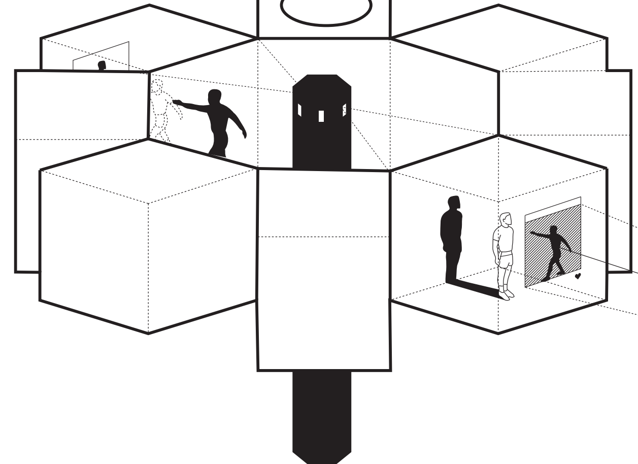
8 Information Retrieval
