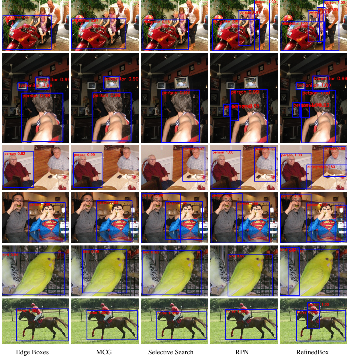
Figure 5: Qualitative comparison for object detection using only top 10 proposals. Here, RefinedBox uses Edge Boxes [9] as the input. All images are from VOC2007 test set.
