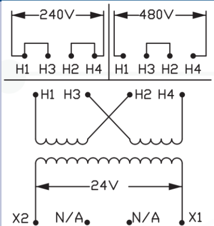
Wiring Diagram D
