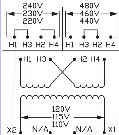
Wiring Diagram C
