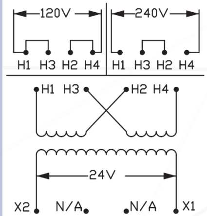
Wiring Diagram B
