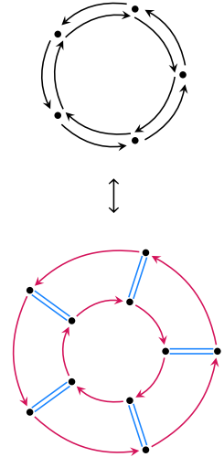
FIGURE 8.1: How a bidirectional 5-cycle corresponds to a dihedral bicycle of degree 5. The doubled bluebell lines indicate that b swaps the two endpoints.
