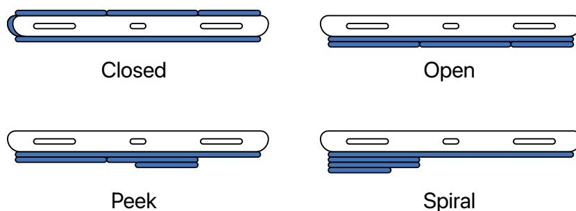
Figure 5-17 Case configurations
