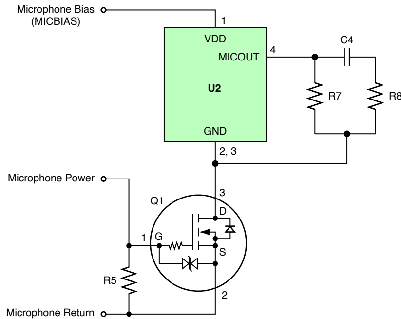
Figure 60-2 Microphone circuit
