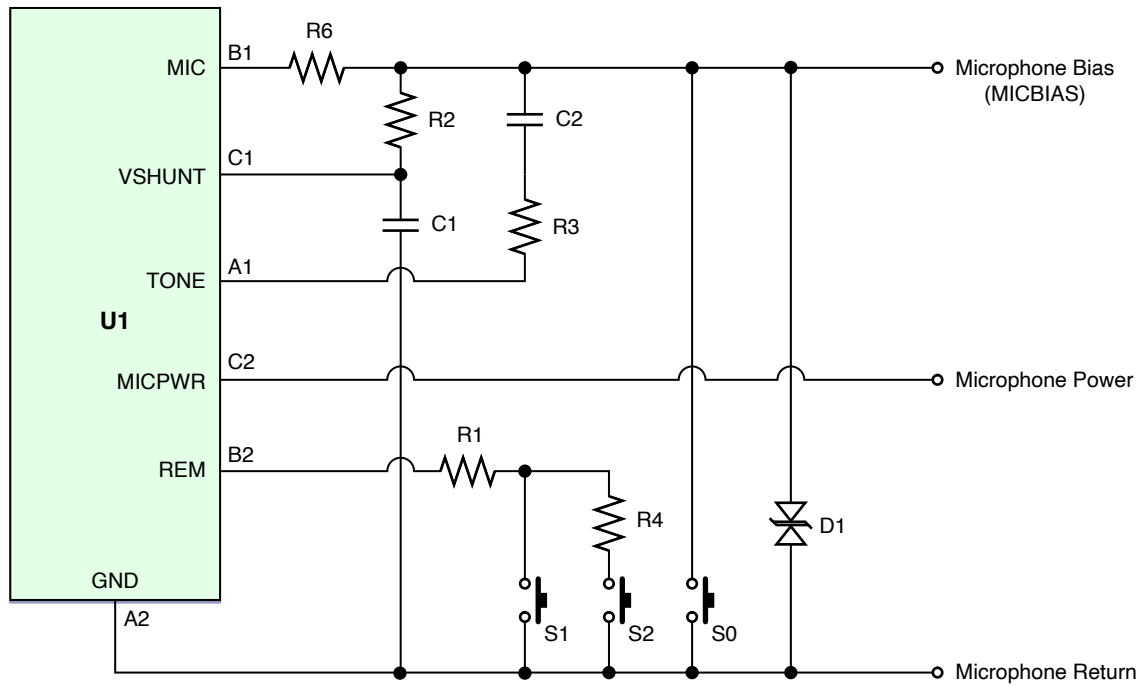
Figure Transmitter circuit 60-1
