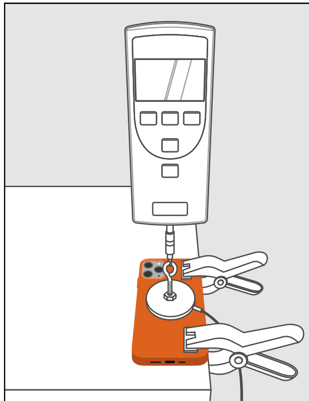
Figure Magnetic force test setup 42-13
