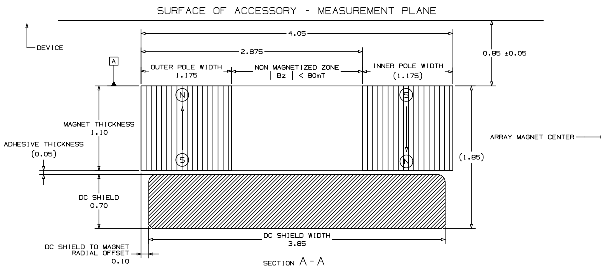
Figure 42-8 MagSafe magnet ring dimensions and polarity
