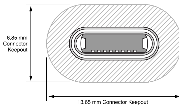
Figure 5-3 Lightning Receptacle (C37) keep-out
