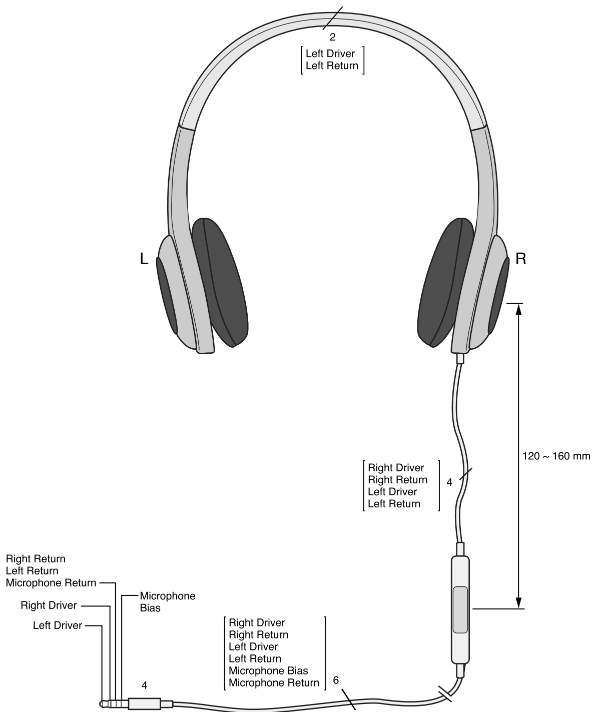
Figure 64-3 Headset plug (3.5 mm), single built-in cable
