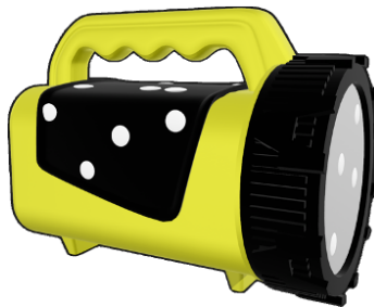
Figure 20-10 Example flashlight USDZ asset showing LED blob primitives (about 10 mm spheres) at the surface where each LED emits light
