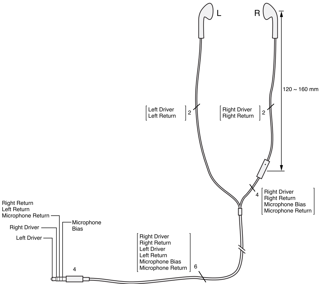
Figure 64-5 Headset plug (3.5 mm), split built-in cable
