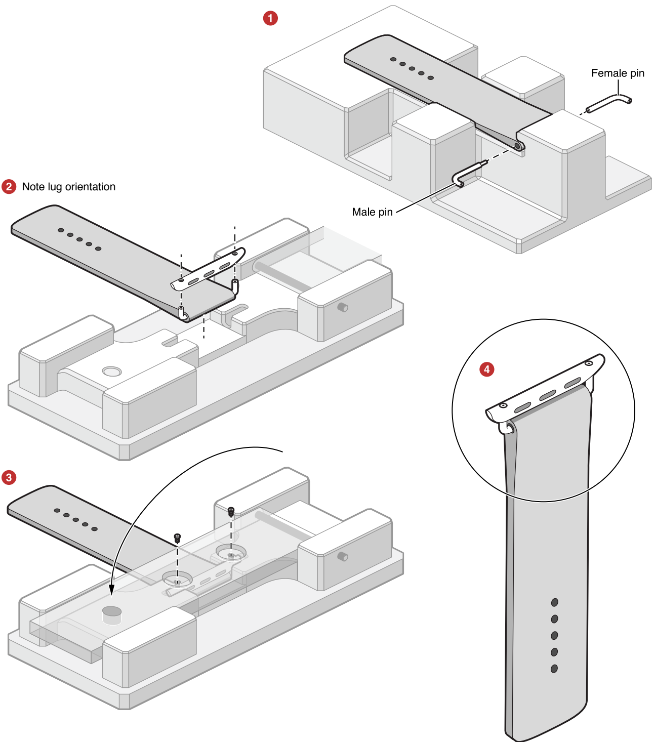
Figure Apple Watch lug assembly fixture 21-1
