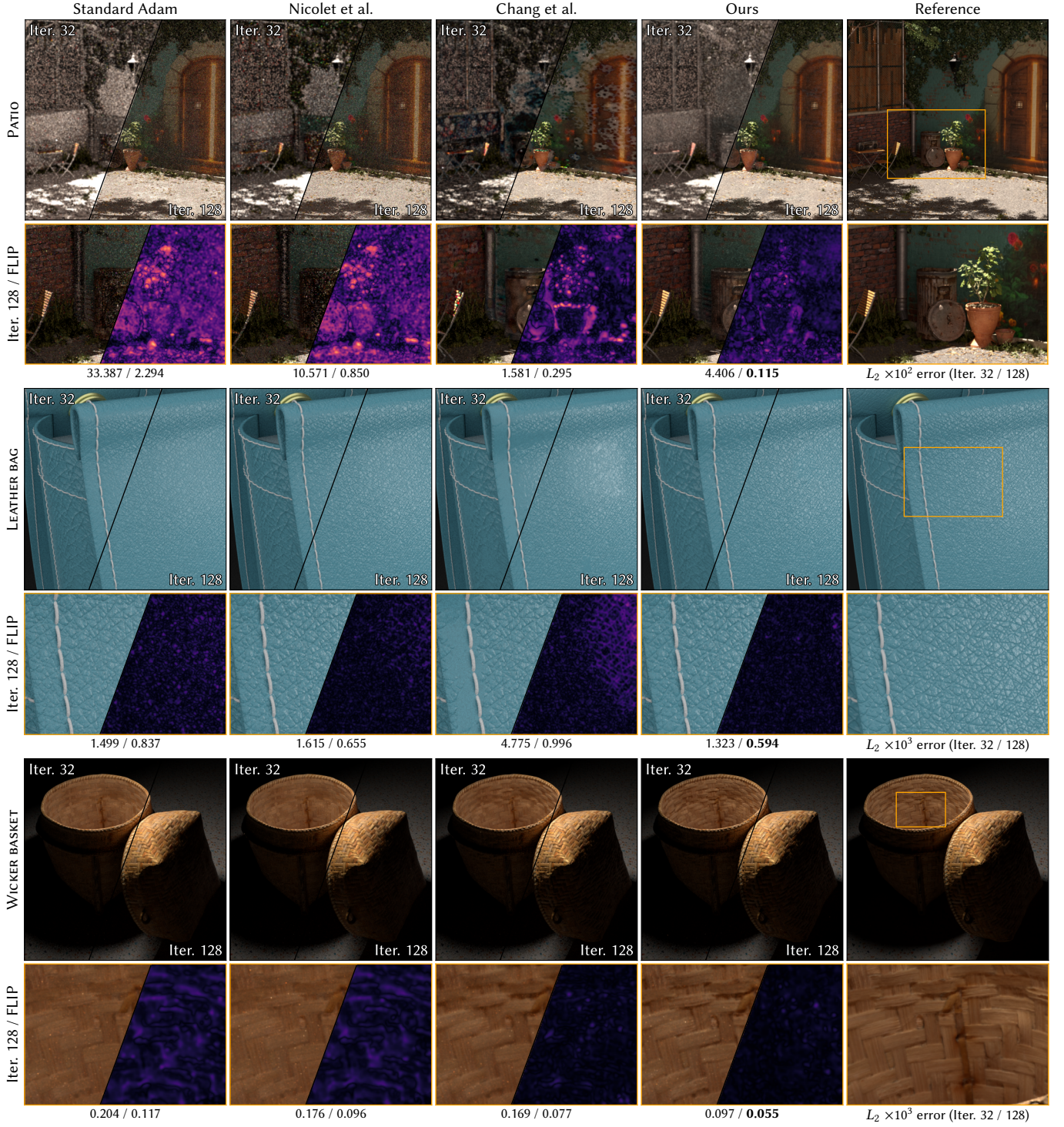
Fig. 7. We compare our method, Laplacian preconditioning [Nicolet et al. 2021] and cross-bilateral gradient filtering [Chang et al. 2024], and visualize FLIP error [Andersson et al. 2020]. We report the L_2 error for the full image after 32 and 128 iterations.
