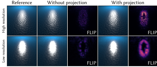
Fig. 8. We render a high-frequency normal map with constant roughness at a 1024^2 and 32^2 render resolution, respectively, and optimize textured roughness ( 2048^2 ) and normal map ( 4096^2 ). We show results with and without projection (i.e., rebuilding of the Laplacian pyramid) at every iteration.
