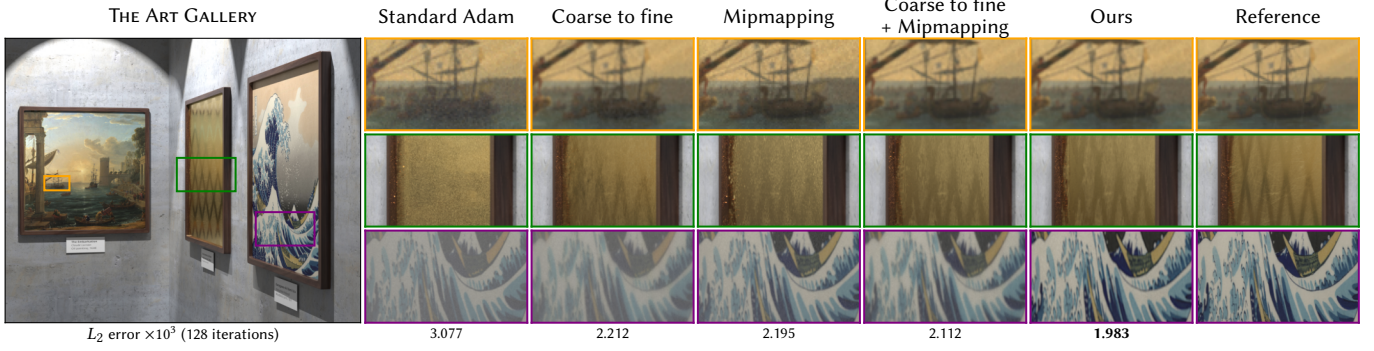
Fig. 3. Comparison of Laplacian mipmapping to existing approaches. We compare our method to standard Adam, coarse-to-fine texture upsampling, differentiable mipmapping and the combination of coarse to fine and mipmapping. From left to right, we optimize each painting’s texture of the following type and resolution: albedo ( 2048^2 ), roughness ( 4096^2 ) and albedo ( 8192^2 ). The rendering resolution is 1500 \times 1200 .
