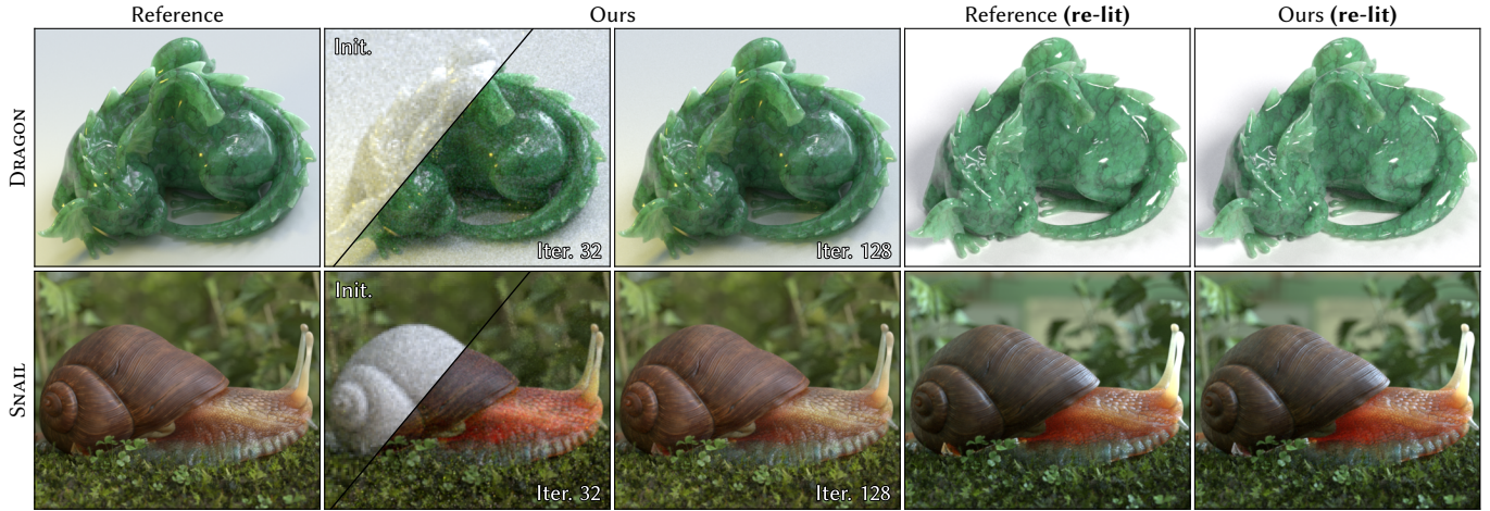
Fig. 14. Inverse rendering of subsurface scattering albedo texture, spectrally-varying extinction and phase-function parameters. On the SNAIL scene, only the shell and skin of the snail are optimized.
