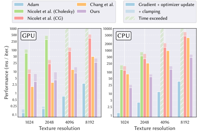
Fig. 6. We plot the time for differentiable forward evaluation, gradient computation, and, if applicable, clamping for our method and prior work over varying texture resolutions. For Nicolet et al. [2021] we show timings for both the original Cholesky solver and our conjugate gradient (CG) solver. The Cholesky solver's preprocessing time is not included in the plot. At 4096^2 , it exceeds 10 min and we therefore only report timings up to 2048^2 .
