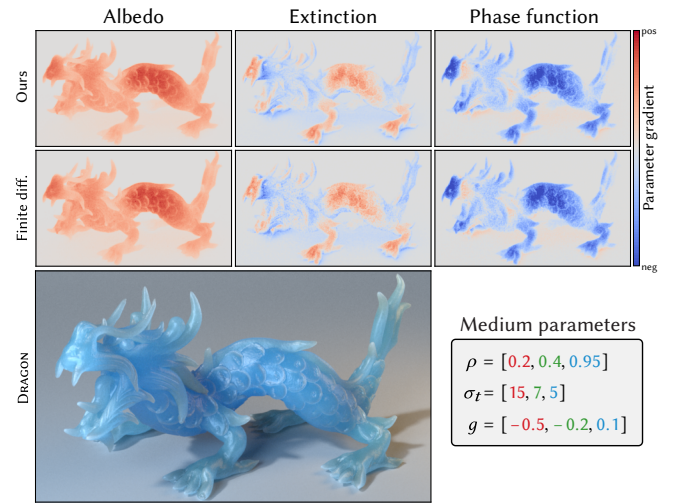
Fig. 11. We validate our implementation’s forward-mode gradients for spectrally-varying albedo, extinction and Henyey-Greenstein phase function anisotropy g against finite differences.
