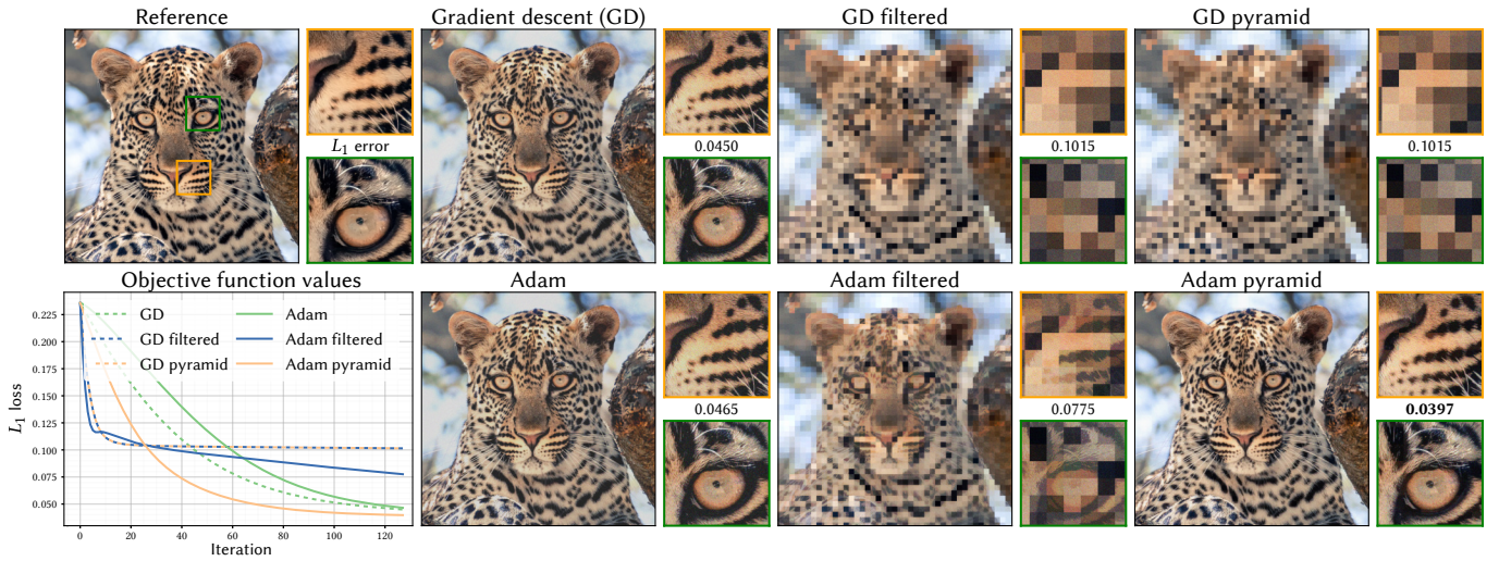
Fig. 4. Optimization of an image that is “rendered” by querying a texture on a regular grid of the same size. Top row: Unmodified gradient descent on a two-level pyramid is equivalent to linearly filtering the gradients of a regular non-pyramid texture. Bottom row: In contrast, the Adam optimizer improves results for the pyramid by adjusting the learning rate per texel per level . For completeness, we also provide results for unmodified gradient descent and Adam.
