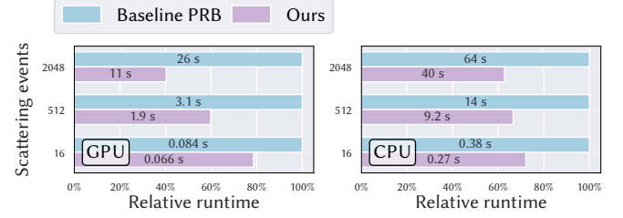
Fig. 10. Performance of our methods when differentiating textured albedo, extinction and phase function (texture resolution of 1024^2 , render resolution of 512^2 , 1 sample per pixel). The horizontal axis is the relative runtime compared to the baseline PRB, and the numbers in each bar are absolute timings. We render three sets of medium parameters, each corresponding to a different average number of scatterings events along a path.
