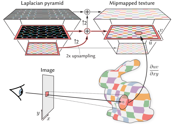
Fig. 2. We construct a texture’s mipmap hierarchy from a Laplacian pyramid. A texture lookup during rendering thus accumulates information from all levels in the Laplacian pyramid below the queried mipmap level (red).
