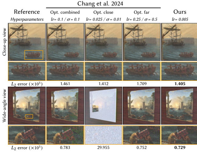
Fig. 5. Comparison of our method to cross-bilateral gradient filtering [Chang et al. 2024] on a scene where a 4096^2 texture is simultaneously optimized for a close-up (top row) and a wide-angle view (bottom row), each rendered at 1024^2 . We find the optimal learning rate ( lr ) and cross-bilateral filter weight \sigma using a grid search. We do this for both views at the same time ("Opt. combined"), as well as for each view individually ("Opt. close" and "Opt. far"). The optimal parameters for one view do not generalize to the other, and even the best combined filter bandwidth \sigma cannot simultaneously handle both views.
