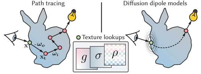
Fig. 9. Left: Path-traced subsurface scattering estimates outgoing radiance by sampling a light path through the object's interior. The medium parameters are set by evaluating 2D textures at the point of entry. Right: An alternative, approximate solution are diffusion dipole models [Jensen et al. 2001], which directly sample outgoing surface locations according to a two-dimensional scattering profile [King et al. 2013].
