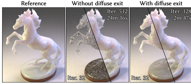
Fig. 12. Impact of using a diffuse exit BSDF on inverse rendering. Left: The reference is rendered without diffuse exit. Center: Unbiased rendering without diffuse exit needs 512 iterations to converge due to the high rendering noise. Right: Our optimization with diffuse exit manages to closely approximate the reference within 128 iterations, and leads to lower variance and render times. Both final optimization states are rendered at a higher sample count to better showcase the quality difference. The reported timings are for the entire optimization.
