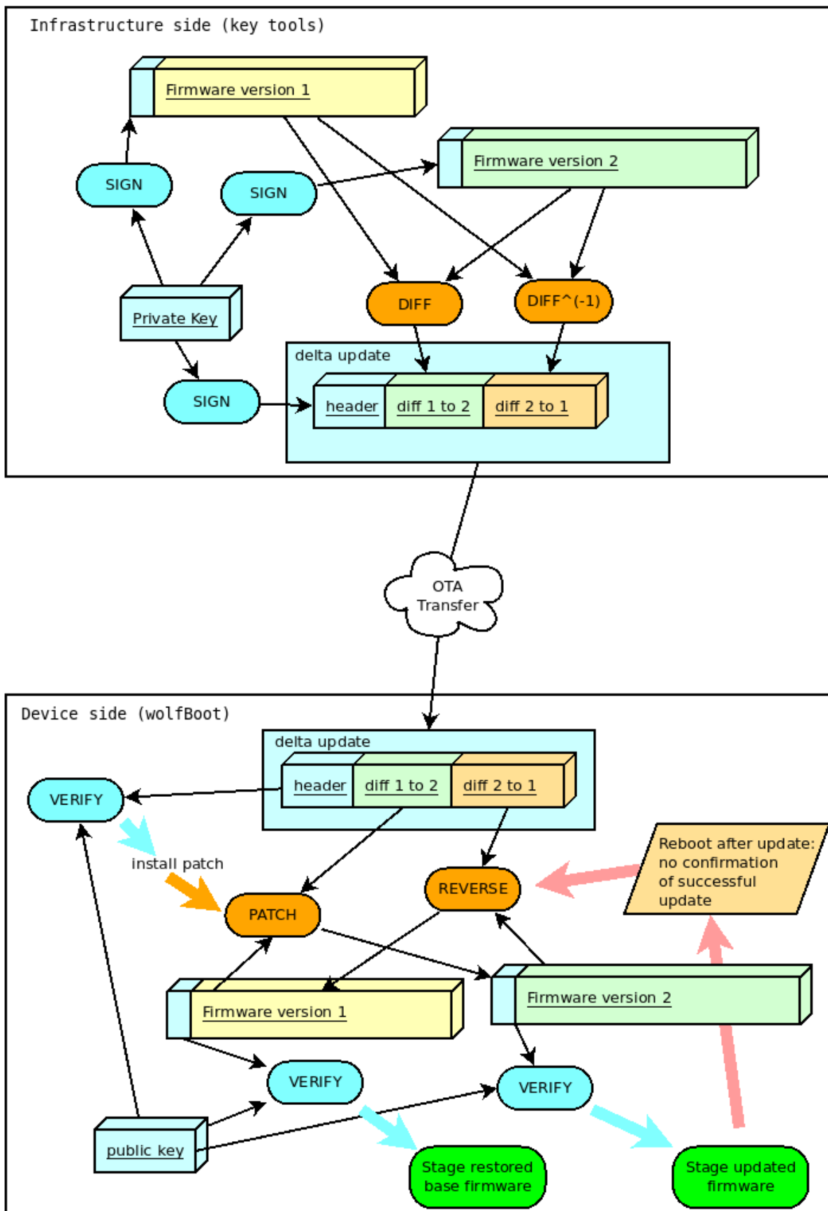
Figure 6: Delta update: details
