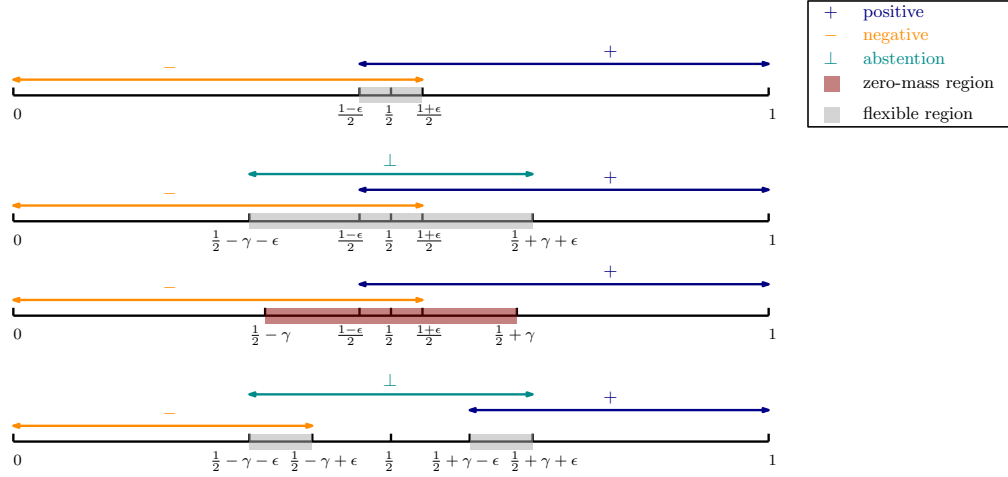
Figure 2.1: Illustration of decision regions under different error criteria. Top : standard excess error \text{err}(\hat{h}) - \text{err}(h^*) . Second : Chow's excess error \text{err}_\gamma(\hat{h}) - \text{err}(h^*) . Third : standard excess error \text{err}(\hat{h}) - \text{err}(h^*) under Massart noise condition with parameter \gamma . Bottom : Chow's excess error relative to the optimal abstaining classifier, i.e., \text{err}_\gamma(\hat{h}) - \inf_{h: X \rightarrow \{0,1,\perp\}} \text{err}_\gamma(h) . In this figure, positive corresponds to predicting label 1 and negative to predicting label 0.
