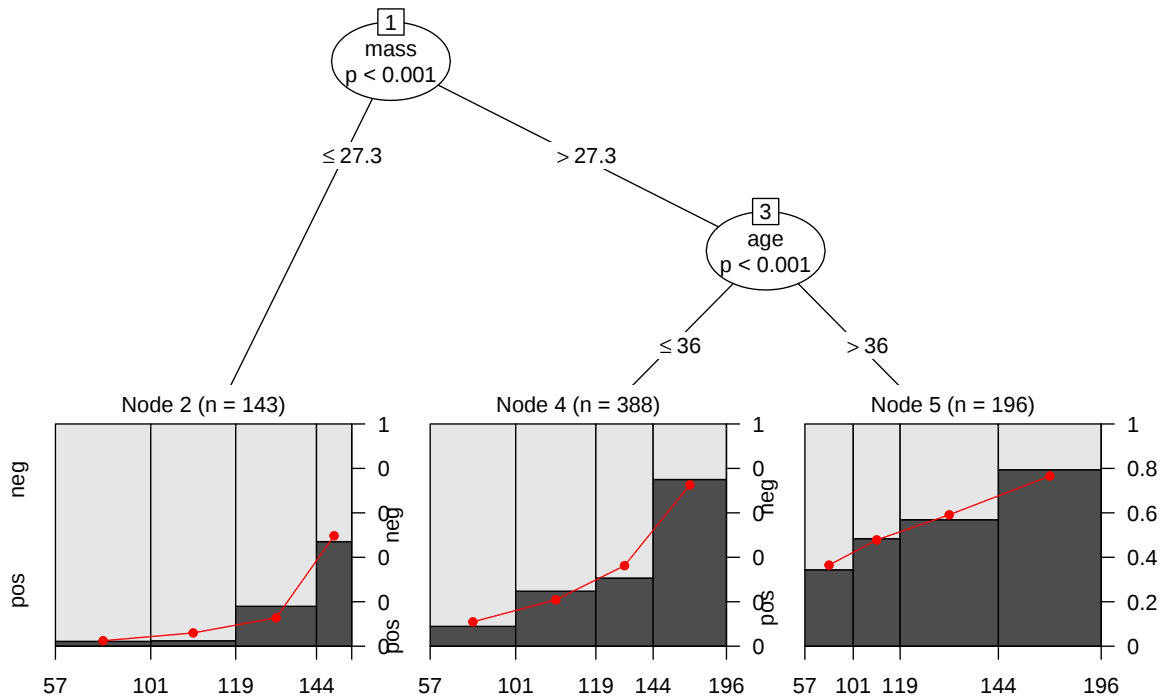
Figure 2: Logistic-regression-based tree for the synthetic diabetes data. The plots in the leaves give spinograms for diabetes versus glucose .
