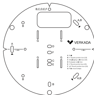
Mounting template
