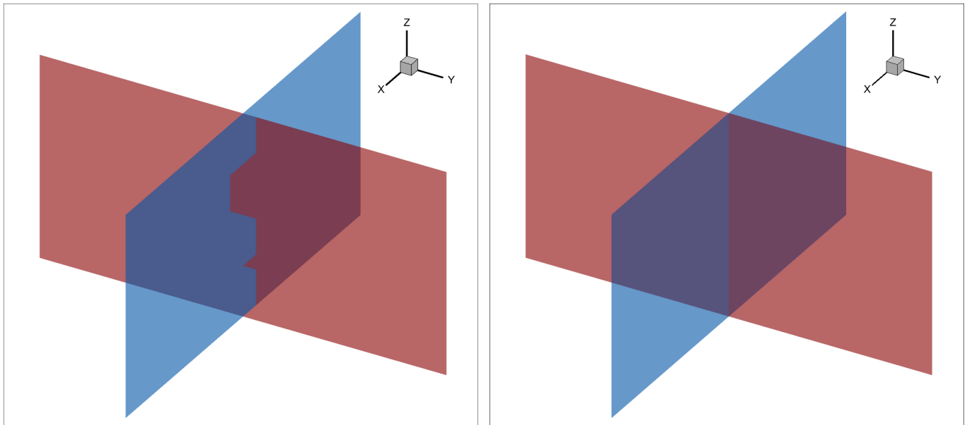
Figure 1. Comparison between transparency in previous versions of Tecplot Focus (left) and with the new GPU-accelerated OIT technique (right). Note how the previous ordering method could cause intersecting surfaces to be incorrectly represented.
