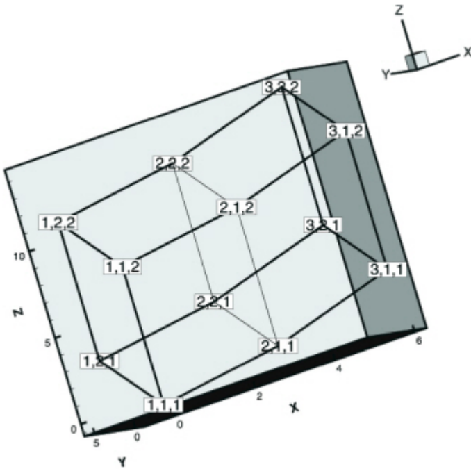
Figure 20. An IJK-ordered data set.
