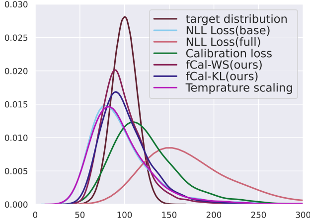
(a) Object detection - Cityscapes[5] - chisquared distribution plots of different baselines. To quantitatively understand the results, see W-dist(q) and KLD(q) rows of table VI. Lower values correspond to better curves, which can be visually understood in the figure.
