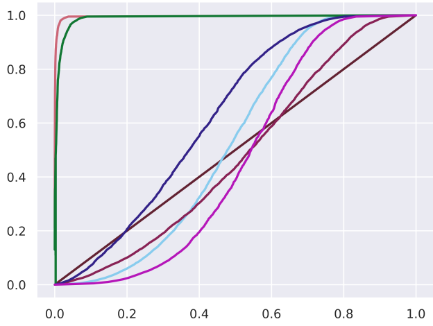
(c) Object detection - Kitti[12] - chisquared reliability diagrams of different baselines. To quantitatively understand the results, see \mathbf{MCE(q)} and \mathbf{ECE(q)} rows of table IV. Lower values reflect better curves.
