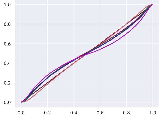
(d) Object detection - Cityscapes[5] - standard normal reliability diagrams of different baselines. To quantitatively understand the results, see MCE(z) and ECE(z) rows of table VI.
