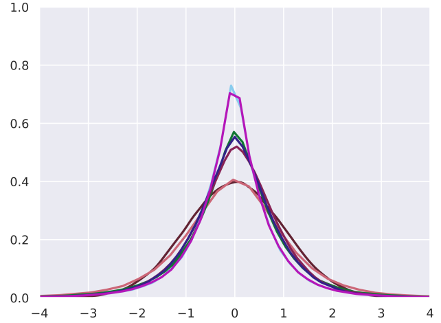
(b) Object detection - Cityscapes[5] - standard normal distribution plots of different baselines. To quantitatively understand the results, see W-dist(z) and KLD(z) rows of table VI.
