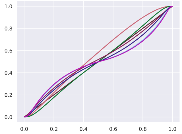
(d) Object detection - Kitti[12] - standard normal reliability diagrams of different baselines. To quantitatively understand the results, see \mathbf{MCE(z)} and \mathbf{ECE(z)} rows of table IV.
