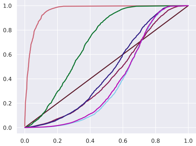
(c) Object detection - Cityscapes[5] - chisquared reliability diagrams of different baselines. To quantitatively understand the results, see MCE(q) and ECE(q) rows of table VI. Lower values reflect better curves.
