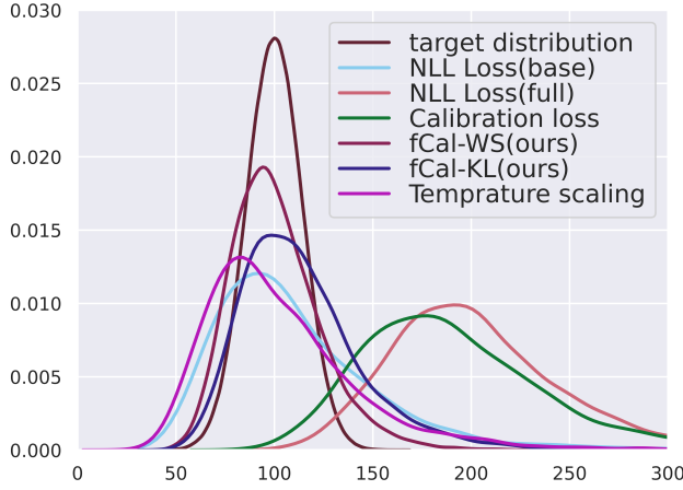
(a) Object detection - Kitti[12] - chisquared distribution plots of different baselines. To quantitatively understand the results, see \mathbf{W-dist(q)} and \mathbf{KLD(q)} rows of table IV. Lower values correspond to better curves, which can be visually understood in the figure.
