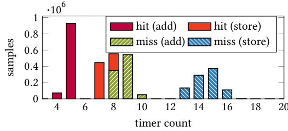
(a) AMD RX 6800 XT
