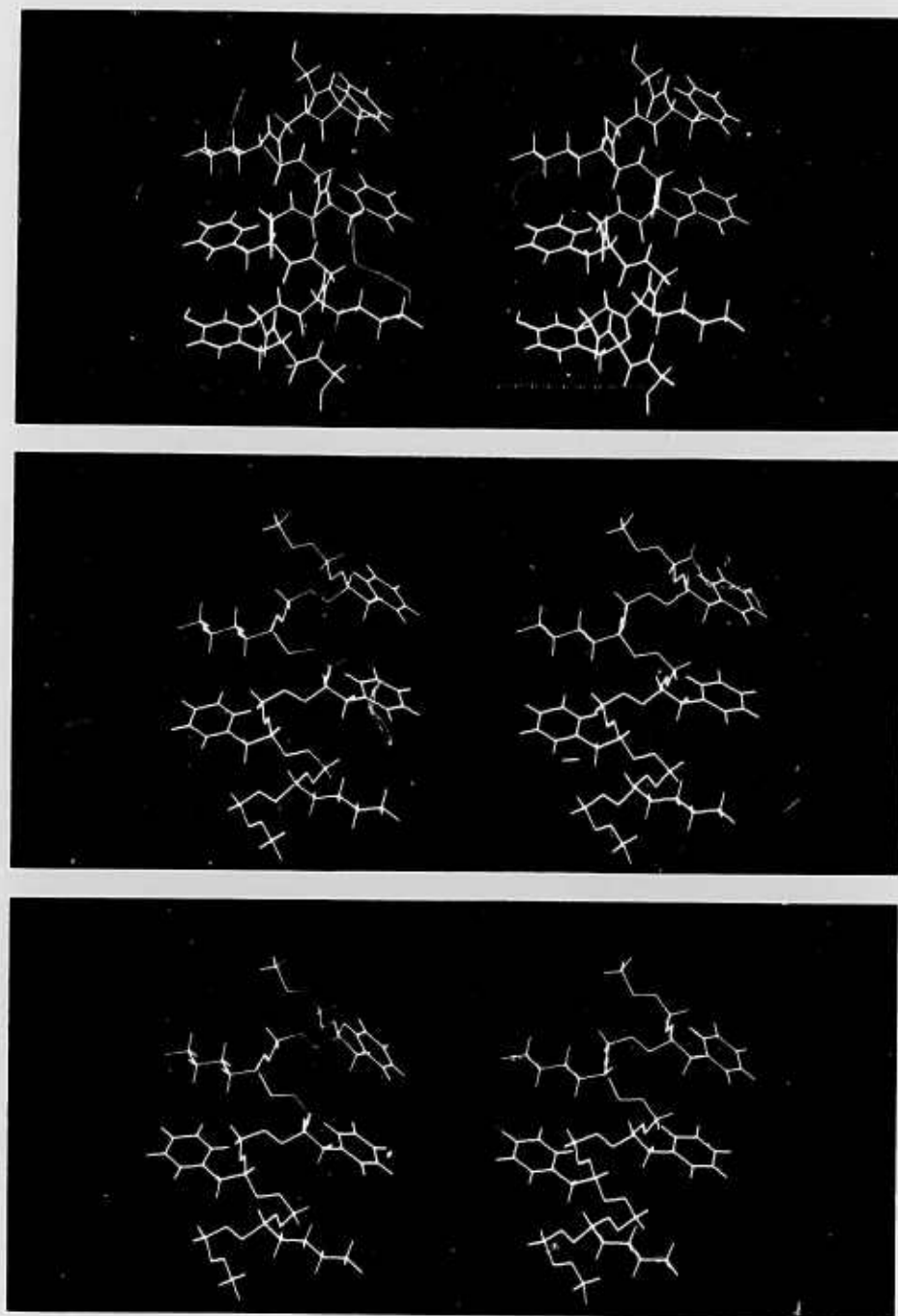
Figure 2. Stereo Pairs of a Protein Molecular Structure
