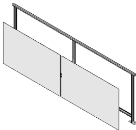
(118.75'') 55.375 x 34.625 FlexRail Infill (Frosted 2 sides)(2 per)
