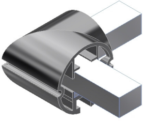
FlexRail Corner Connector Set (2 Set Screws per Connection) Part # Corner Connector
