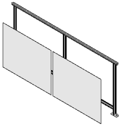
(93") 42.5 x 34.625 FlexRail Infill (Frosted 2 sides)(2 per) Part # 40-45
