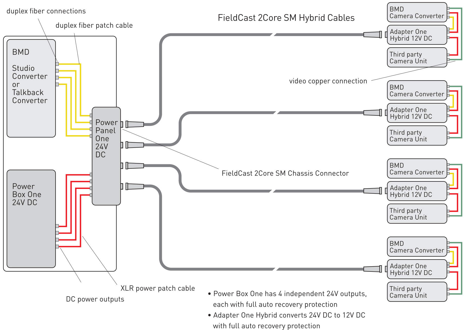
figure 8: FieldCast setup with Power Box One, Power Panel One, and Adapter One Hybrid
