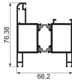
JY-HOPO-010 + JY-HOPO-009 upper and lower frame Weight : 1.09 kg/m , 0.903 kg/m
