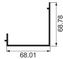
WB150-21 sink Weight : 0.84 kg/m
