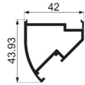
JY-42ZD-10 corners Weight : 0.743 kg/m
