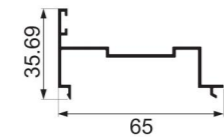
JY-75ZD-04 closing 1 Weight : 0.441 kg/m
