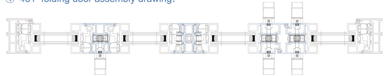
④ 431 folding door assembly drawing:
