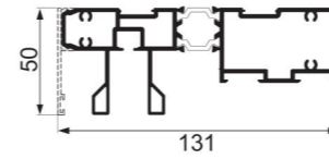
JNW-GD925F lifting top rails Weight : 2.62 kg/m
