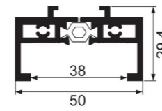
WB150-A6 horizontal top frame Weight : 1.06 kg/m
