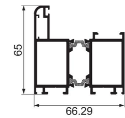
JY-HOPO-008 + JY-HOPO-007 door frame Weight : 1.04 kg/m , 0.847 kg/m
