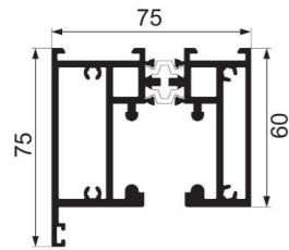
JY75ZD-24 + JY75ZD-25 hanging rail Weight : 1.890 kg/m , 1.520 kg/m
