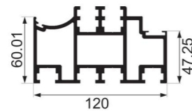
JY-120-08 small center column Weight : 5.143 kg/m
