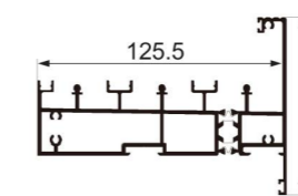
JNW-CT1460F three-track suspended bottom rail Weight : 3.07 kg/m
