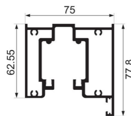
JY-75ZD-10 hanging rail Weight : 2.804 kg/m
