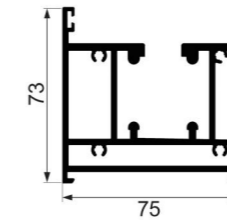
JY-75ZD-28 hanging rail Weight : 3.210 kg/m
