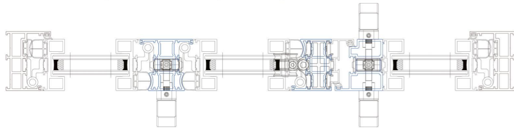
② 321 folding door assembly drawing:
