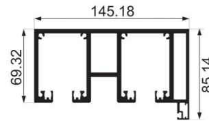
JY-120-01 hanging rail Weight : 6.582 kg/m
