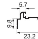
JY-42ZD-06 closing Weight : 0.15 kg/m
