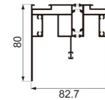
JNW-CT1487F two-track suspended upper rail Weight : 2.32 kg/m
