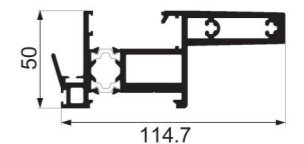
JNW-SJC33 strengthen glass door with hook Weight : 3.58 kg/m
