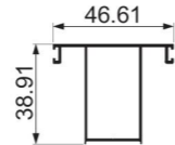
JNW-XT1331 side frame double cover Weight : 0.46 kg/m
