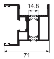
WB150-C8 90 degree corner vertical sealing frame Weight : 2.2 kg/m
