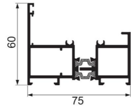
JY-HOPO-012 + JY-HOPO-013 lower rail Weight : 0.935 kg/m , 0.767 kg/m
