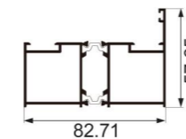
JNW-CT1420F two-track side frame transform Weight : 1.40 kg/m
