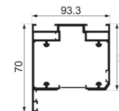
JY-42ZD-02 upper track/outframe Weight : 1.661 kg/m
