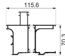
JNW-SJC28A 150 side frame transform Weight : 3.29 kg/m
