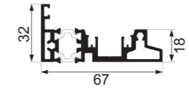
JY-58DQ-19 + JY-58DQ-20 low track Weight : 0.398 kg/m , 0.826 kg/m
