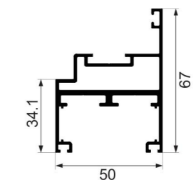
JY-50ZD-12 mullion Weight : 1.3 kg/m
