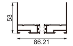
JNW-CT1416F two rail side seal Weight : 1.34 kg/m
