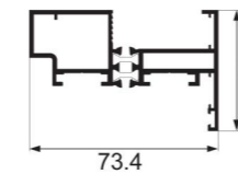
DZ-CT795F slim glass sash Weight : 1.36 kg/m
