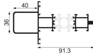
JNW-CT1738F strengthen center column Weight : 2.42 kg/m
