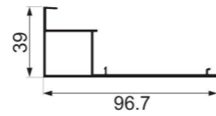
JNW-ZN029 150 side frame cover Weight : 0.8 kg/m
