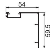
JNW-A-031 112 single vertical door frame with hook Weight : 0.53 kg/m
