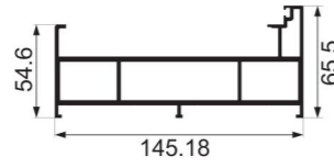
JY-120-02 side frame Weight : 3.715 kg/m
