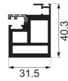
JNW-XT1466F mesh door with hook Weight : 1.17 kg/m
