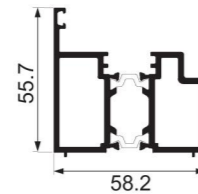
JY58DQ-23 + JY58DQ-24 door frame closing Weight : 0.879 kg/m , 0.765 kg/m
