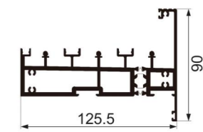
JNW-CT1708F 3.0 three-track suspended bottom rail Weight : 3.87 kg/m
