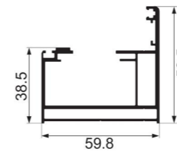
YC-SZ-6001 60 side frame Weight : 1.251 kg/m
