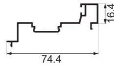
JY-75ZD-05 closing 2 Weight : 0.506 kg/m
