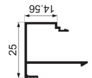
JY-50ZD-10A window pressing line 1 Weight : 0.218 kg/m
