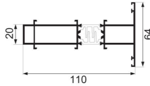
JNW-ZH813A injection molded center post Weight : 1.82 kg/m
