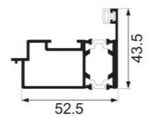
JY-58DQ-29 + JY-58DQ-28 outframe closing Weight : 0.603 kg/m , 0.357 kg/m
