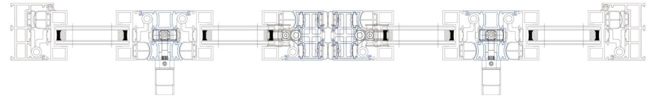
⑤ 422 folding door assembly drawing:
