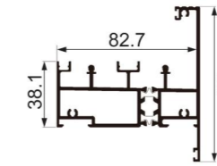
JNW-CT1459F two-track suspended bottom rail Weight : 2.29 kg/m
