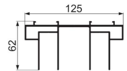
JNW-XT864 intelligent two-rail additional rail Weight : 2.18 kg/m
