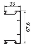
JNW-A-028 70 double vertical door frame with hook Weight : 0.66 kg/m
