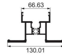
WB150-C7 double openable vertical sealing frame Weight : 3.1 kg/m
