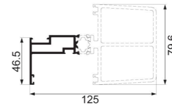
JNW-SJC14 strengthen inner frame Weight : 3.98 kg/m
