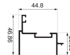
JY-50ZD-04 outframe closing Weight : 0.588 kg/m
