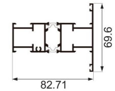
JNW-CT1343G two rail inner frame Weight : 1.54 kg/m
