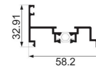
JY-58DQ-25 + JY-58DQ-26 small center column closing Weight : 0.351 kg/m , 0.244 kg/m
