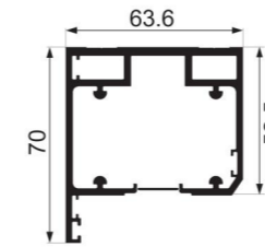
JY-42ZD-19 upper track/outframe Weight : 1.70 kg/m
