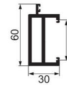
JNW-A-041 30 slim vertical door frame Weight : 1.40 kg/m
