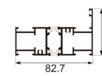
JNW-CT1343E two tracks fixed up and down Weight : 1.49 kg/m
