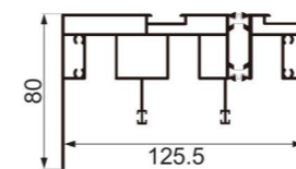
JNW-CT1485F three-track suspended upper rail Weight : 3.04 kg/m
