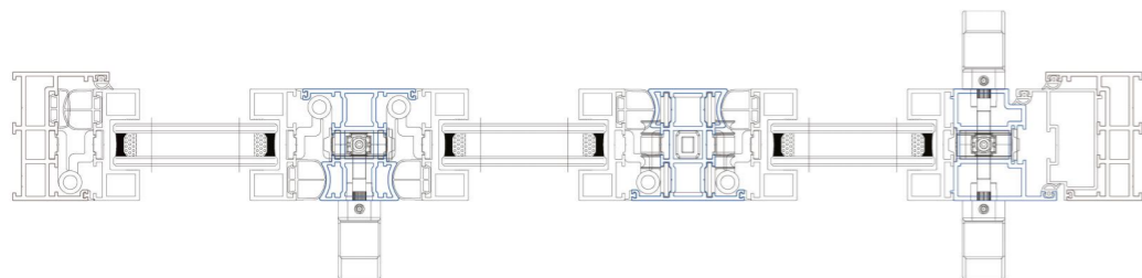
③ 330 folding door assembly drawing:
