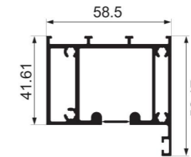
JY-50ZD-05 hanging rail Weight : 1.6 kg/m
