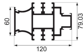
JY-120-07 big center column Weight : 5.163 kg/m
