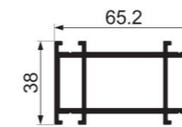
JY-75ZD-26 even-numbered central column Weight : 1.740 kg/m
