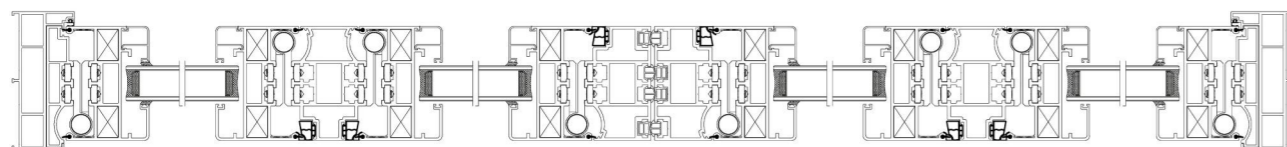
⑤ 422 folding door assembly drawing:
