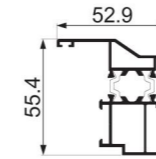
HC110 sash center frame Weight : 1.0 kg/m
