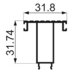
JNW-XT1468 bottom double side frame cover Weight : 0.38 kg/m
