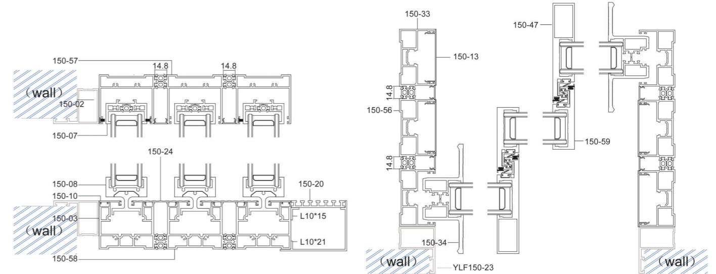
Three-track assembly drawing (can have as many tracks as you like)
