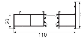
JNW-BK812A injection molded frame Weight : 1.69 kg/m
