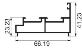
JY-HOPO-006 closing Weight : 0.935 kg/m
