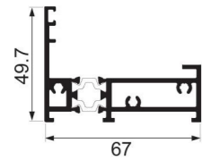
JY-58DQ-14 + JY58DQ-16 big lower rail Weight : 0.590 kg/m , 0.835 kg/m
