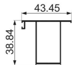
JNW-XT1332F side frame single cover Weight : 0.41 kg/m
