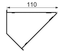
ZJ110B 110 degree corner – 135° Weight : 1.13 kg/m
