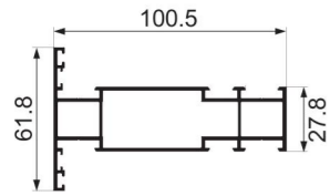
JY-42ZD-14 center column Weight : 1.57 kg/m
