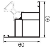
JNW-XT1009 outside the 90° slim corner Weight : 1.14 kg/m
