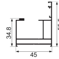
YC-SZ-4501 45 side frame Weight : 0.705 kg/m
