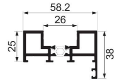
JY-58DQ-03 + JY-58DQ-27 integrated splicing door frame Weight : 0.566 kg/m , 0.642 kg/m
