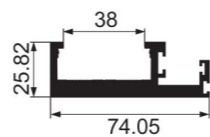
WB150-59 vertical interlock frame Weight : 1.91 kg/m
