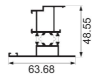
HC235B center frame for glass fans Weight : 1.0 kg/m
