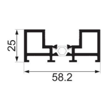
JY-58DQ-03 split splicing door frame Weight : 0.566 kg/m
