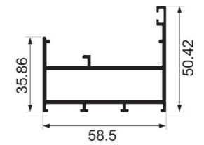
JY-50ZD-01 side frame Weight : 1.06 kg/m
