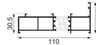
JNW-BK760A outer frame Weight : 1.65 kg/m
