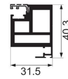
JNW-XT1671 outside mesh door with hook Weight : 1.24 kg/m
