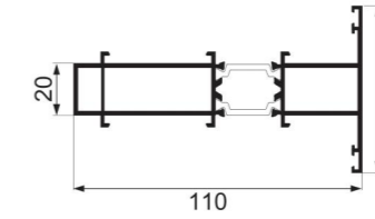
JNW-ZH813A injection molded center post Weight : 1.82 kg/m
