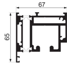
JY58DQ-11 + JY58DQ-12 hanging rail Weight : 0.822 kg/m , 1.965 kg/m
