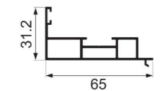
JY-75ZD-31 outframe closing Weight : 0.736 kg/m
