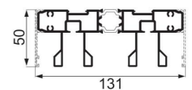
JNW-TS918F lifting two-rail top rail Weight : 2.84 kg/m
