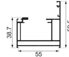
YC-SZ-5001 50 side frame Weight : 1.011 kg/m
