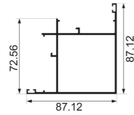
JY-50ZD-15 fixed corner Weight : 1.65 kg/m
