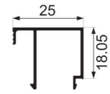
JY-50ZD-13A window pressing line 2 Weight : 0.204 kg/m
