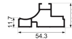
JY-50ZD-02 small outframe Weight : 0.703 kg/m
