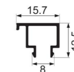
YC-SZ-4503 burclose 1 Weight : 0.114 kg/m
