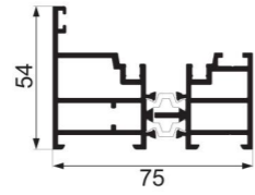
JY75ZD-18 + JY75ZD-19 side frame Weight : 1.430 kg/m , 1.060 kg/m
