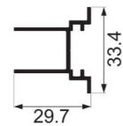
JY-75ZD-03 excipients Weight : 0.370 kg/m
