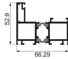
JY-HOPO-003 + JY-HOPO-004 door frame Weight : 0.962 kg/m , 0.725 kg/m
