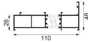
JNW-BK812A injection molded frame Weight : 1.69 kg/m
