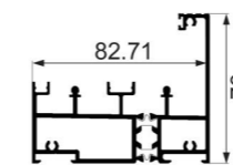
JNW-CT1676F two-track suspended bottom rail(landing) Weight : 2.19 kg/m
