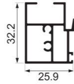
JY-50TS-03 movable door frame with hook Weight : 0.495 kg/m
