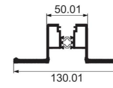
WB150-C5 vertical frame with handle Weight : 2.58 kg/m
