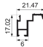
JY-HOPO-014 upper and lower frame auxiliary materials Weight : 0.191 kg/m
