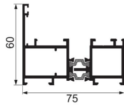
JY-HOPO-001 + JY-HOPO-002 upper rail Weight : 0.974 kg/m , 0.766 kg/m
