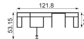
JNW-XT1586 suspended window intelligent upper track additional track Weight : 1.90 kg/m
