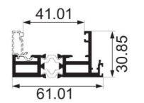
JNW-TS929F inside slim vertical door frame Weight : 1.23 kg/m
