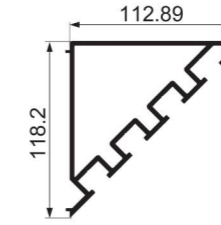
JY-120-12 corner Weight : 3.951 kg/m
