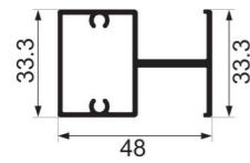
JY-50ZD-16 door frame center column Weight : 0.82 kg/m
