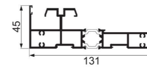
JNW-GD919F lifting bottom rail Weight : 2.48 kg/m
