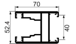
JNW-TS70 70 lifting vertical door frame Weight : 2.26 kg/m
