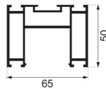
JY-75ZD-08 closing door frame Weight : 1.679 kg/m
