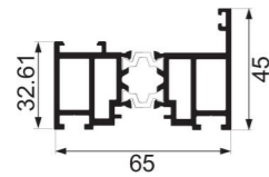
JY75ZD-21 + JY75ZD-20 door frame Weight : 0.845 kg/m , 0.927 kg/m
