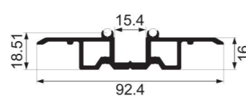
JY-HOPO-011 lower rail Weight : 1.18 kg/m
