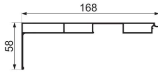
JNW-ZN023 screen cover Weight : 1.71 kg/m
