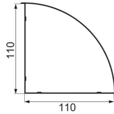
ZJ110A 110 corners – 90° Weight : 1.42 kg/m
