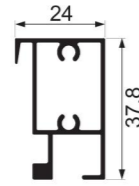
JY-50TS-02 fixed door frame with hook Weight : 0.493 kg/m
