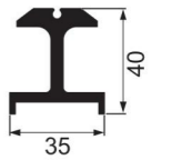
WB150-28 horizontal bottom frame base for roller Weight : 1.16 kg/m
