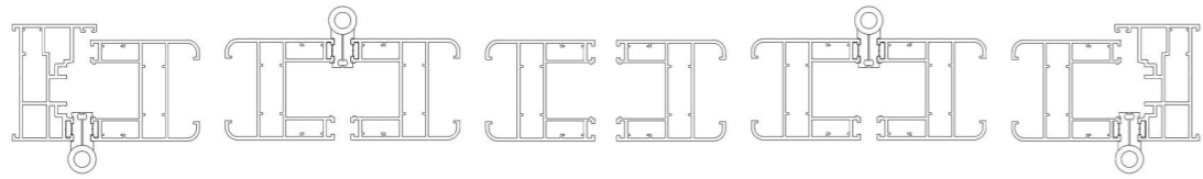
⑤ 431 folding door assembly drawing:
