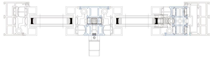
① 220 folding door assembly drawing:
