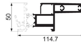
JNW-SJC25 strengthen glass door with hook Weight : 3.72 kg/m
