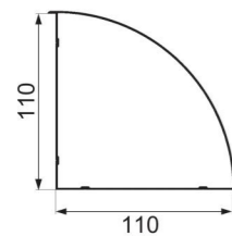
ZJ110A 90 degree corner Weight : 1.35 kg/m
