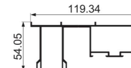
JNW-XT1186 intelligent top rail additional groove Weight : 1.78 kg/m
