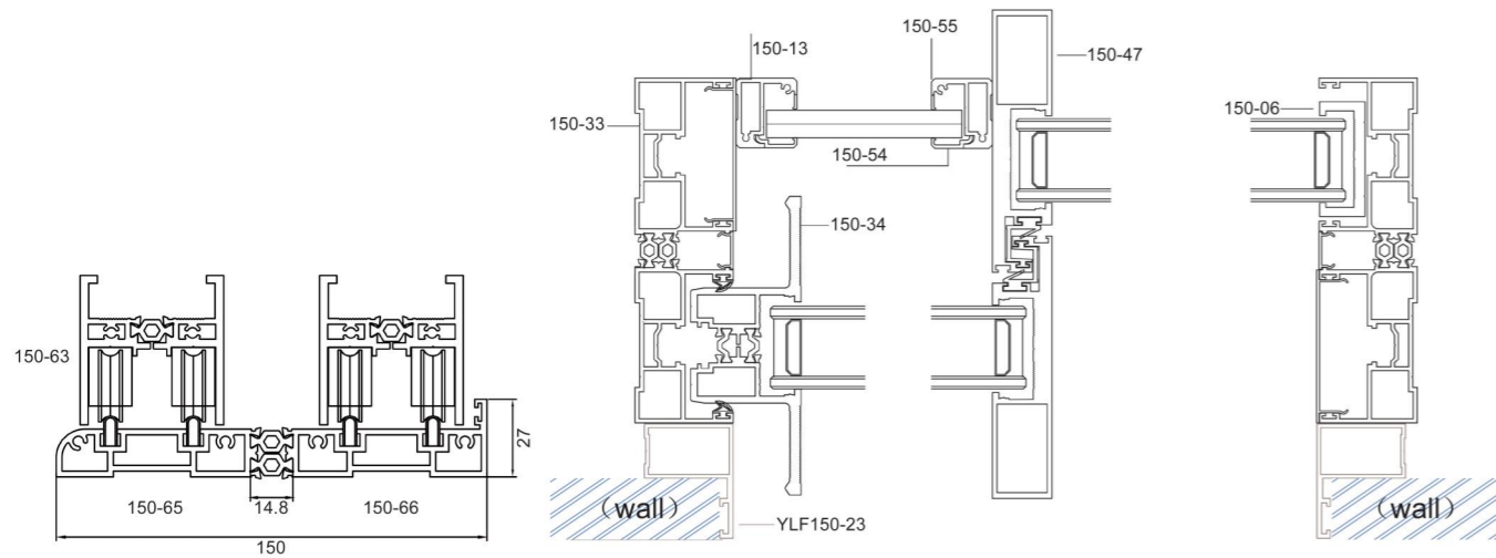
Low rail and below without pre-embedded plan
