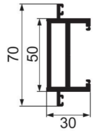
JNW-A-044 30 slim double vertical door frame with hook Weight : 1.35 kg/m
