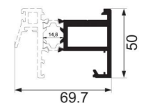
JNW-SJC041 glass door with hook Weight : 2.38 kg/m
