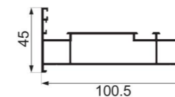
JY-42ZD-15 side frame Weight : 1.377 kg/m
