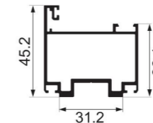
YC-SZ-5002 50 door frame Weight : 0.843 kg/m
