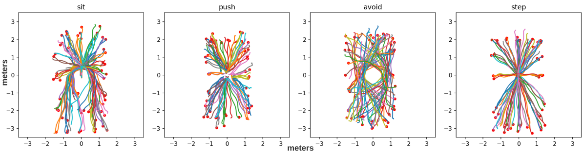
Real-world Dataset:
