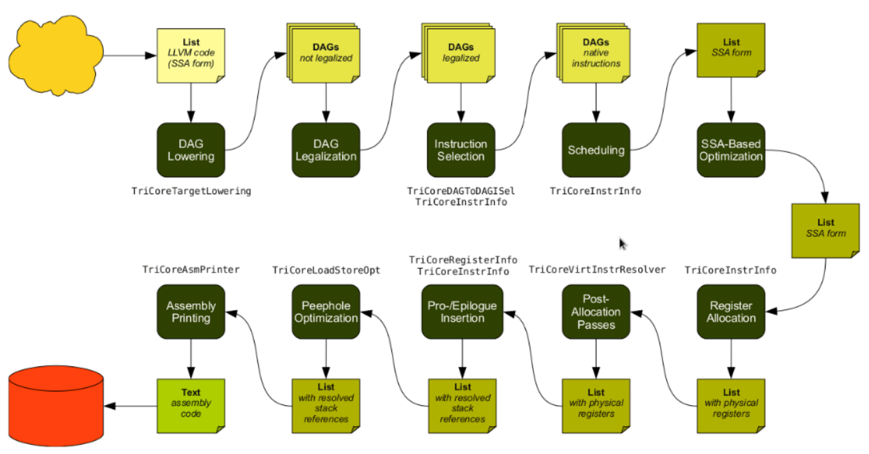
Fig. 2.9: tricore_llvm.pdf : Code Generation Sequence On the path from LLVM code to assembly code, numerous passes are executed, and several data structures are used to represent intermediate results.
