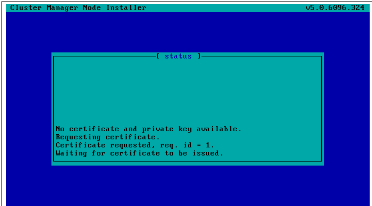
Figure 5.8: Certificate Request
