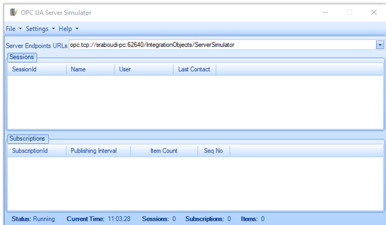
Figure 12: OPC UA Server Simulator - Main User Interface
