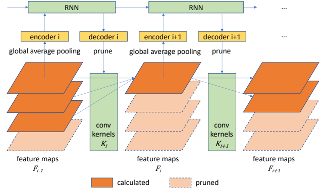
Fig. 2. The overall framework of our RNP. RNP consists of two sub-networks: the backbone CNN network and the decision network. The convolution kernels of backbone CNN network are dynamically pruned according to the output Q-value of the decision network, conditioned on the state forming from the last calculated feature maps.
