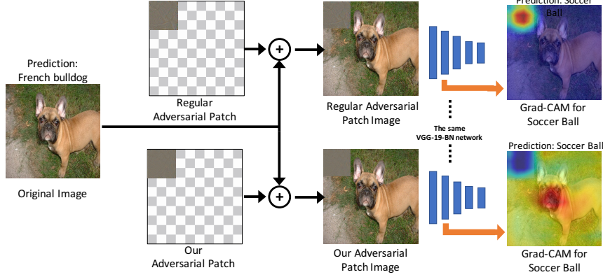
Figure 1: We show that Grad-CAM highlights the patch location in the image perturbed by regular targeted adversarial patches [6] (top row). Our modified attack algorithm goes beyond fooling the final prediction by hiding the patch in the Grad-CAM visualization, making it difficult to investigate the cause of the mistake. Note that Grad-CAM visualizes the cause of target category.
