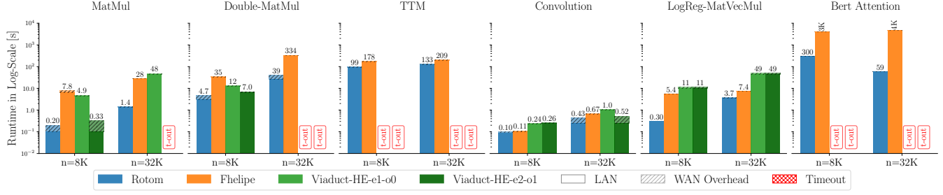
Figure 7: Performance in Log-Scale on OpenFHE for Rotom, Fhelipe, Viaduct-HE. Diagonal hash bars indicate runtimes in the WAN setting with higher communication overheads. t-out indicates the benchmark did not compile within 24hrs.
