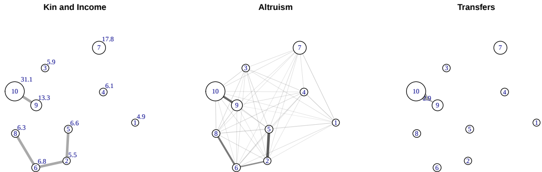
Figure 9: Altruism less noisy: \beta_0 = -1.8, \beta_1 = 2, \underline{\sigma = 0.3}, \kappa = \infty
