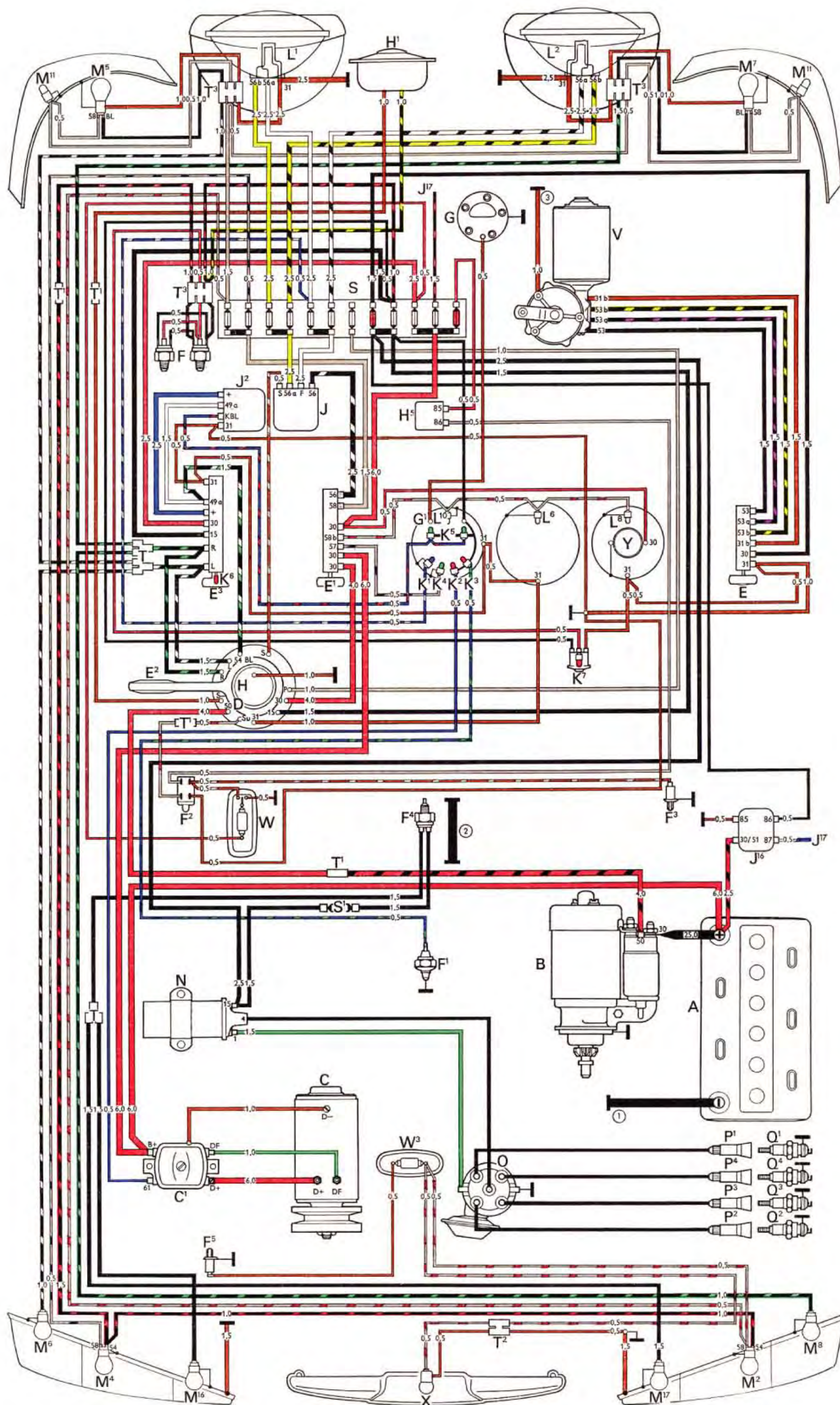
Wiring diagram VW Type 3 – from August 1969
