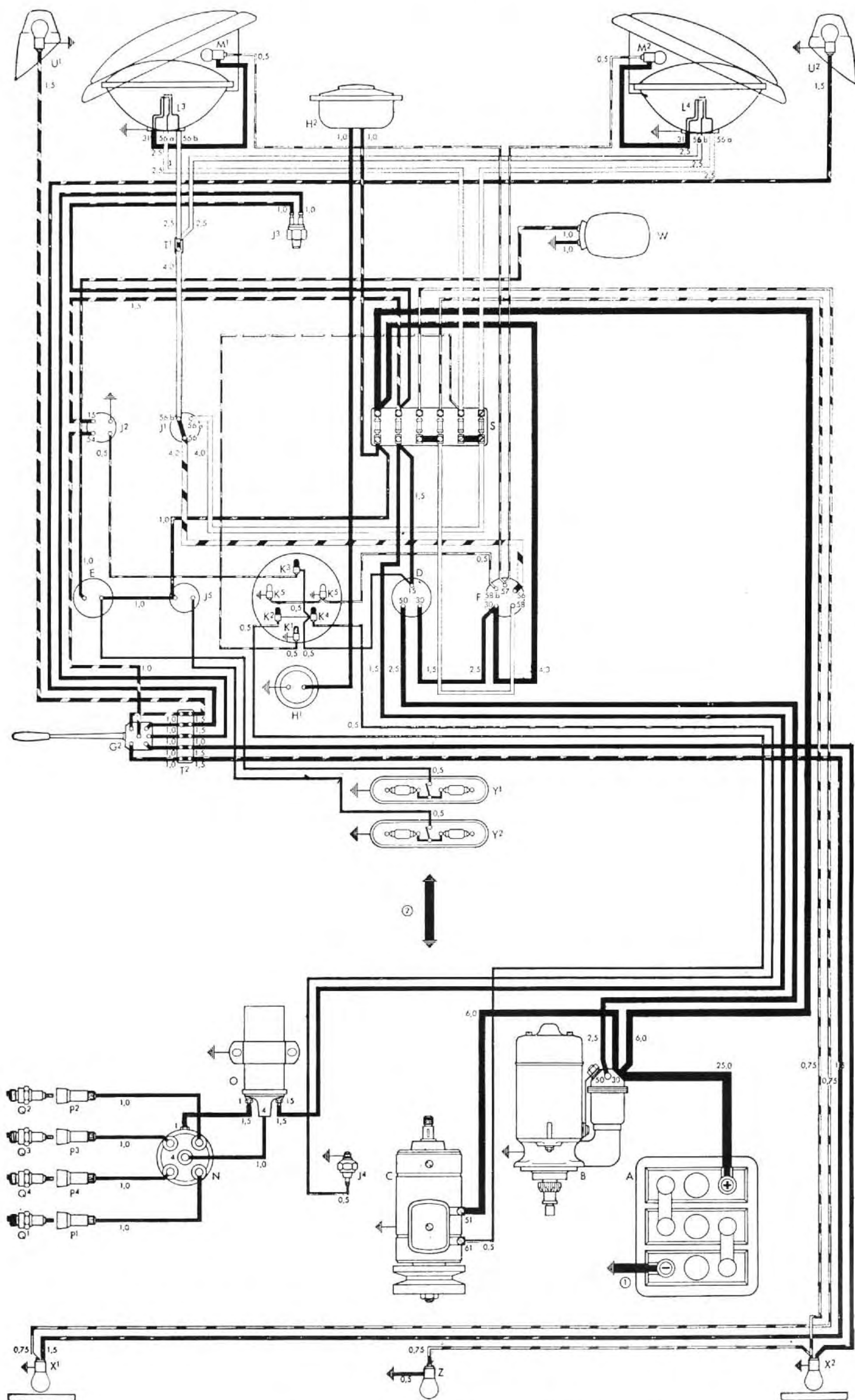
Wiring diagram for the U.S. version of the Transporter.
