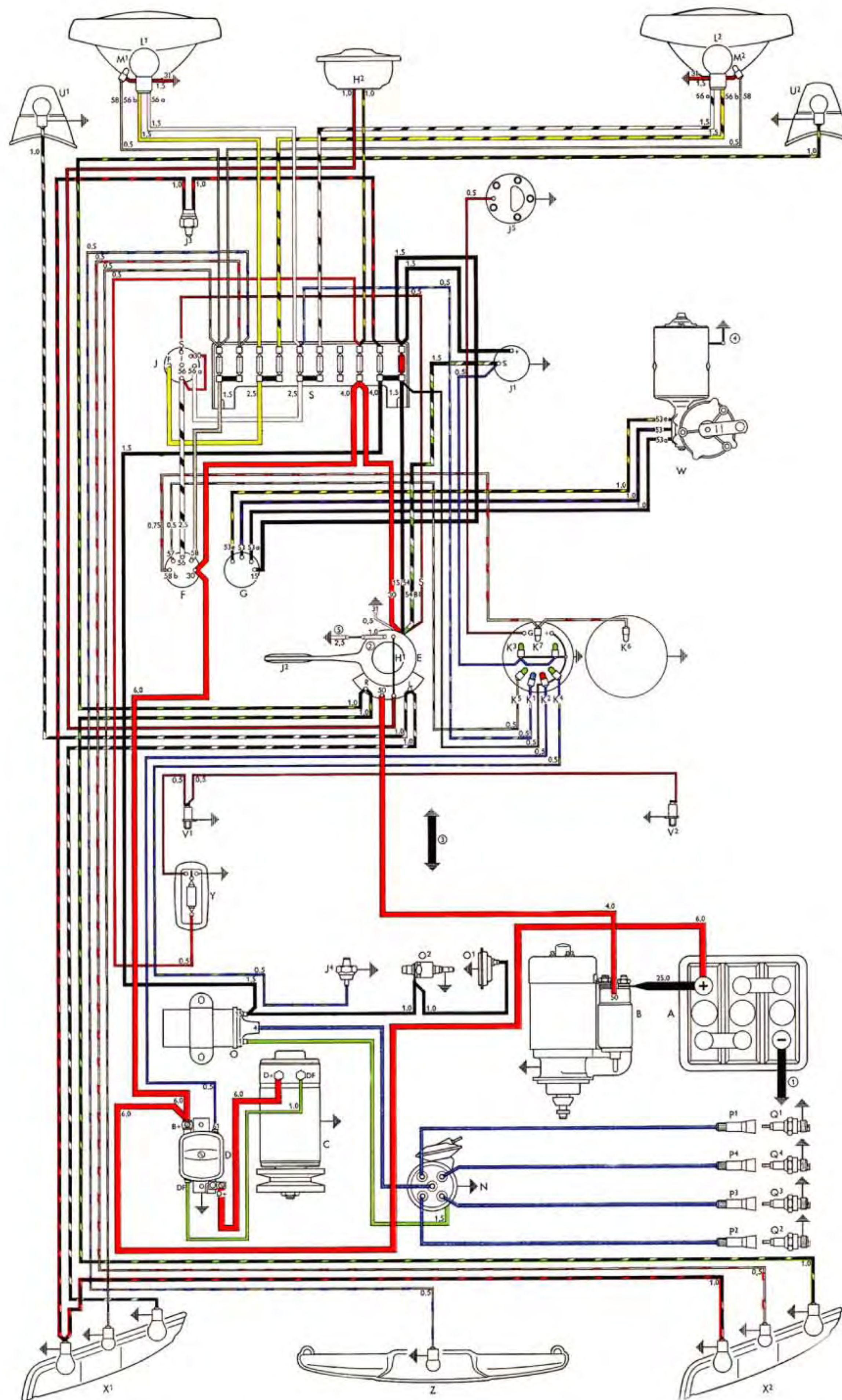
Wiring Diagram VW 1500 N (from August 1963, Chassis No. 0 221 975)
