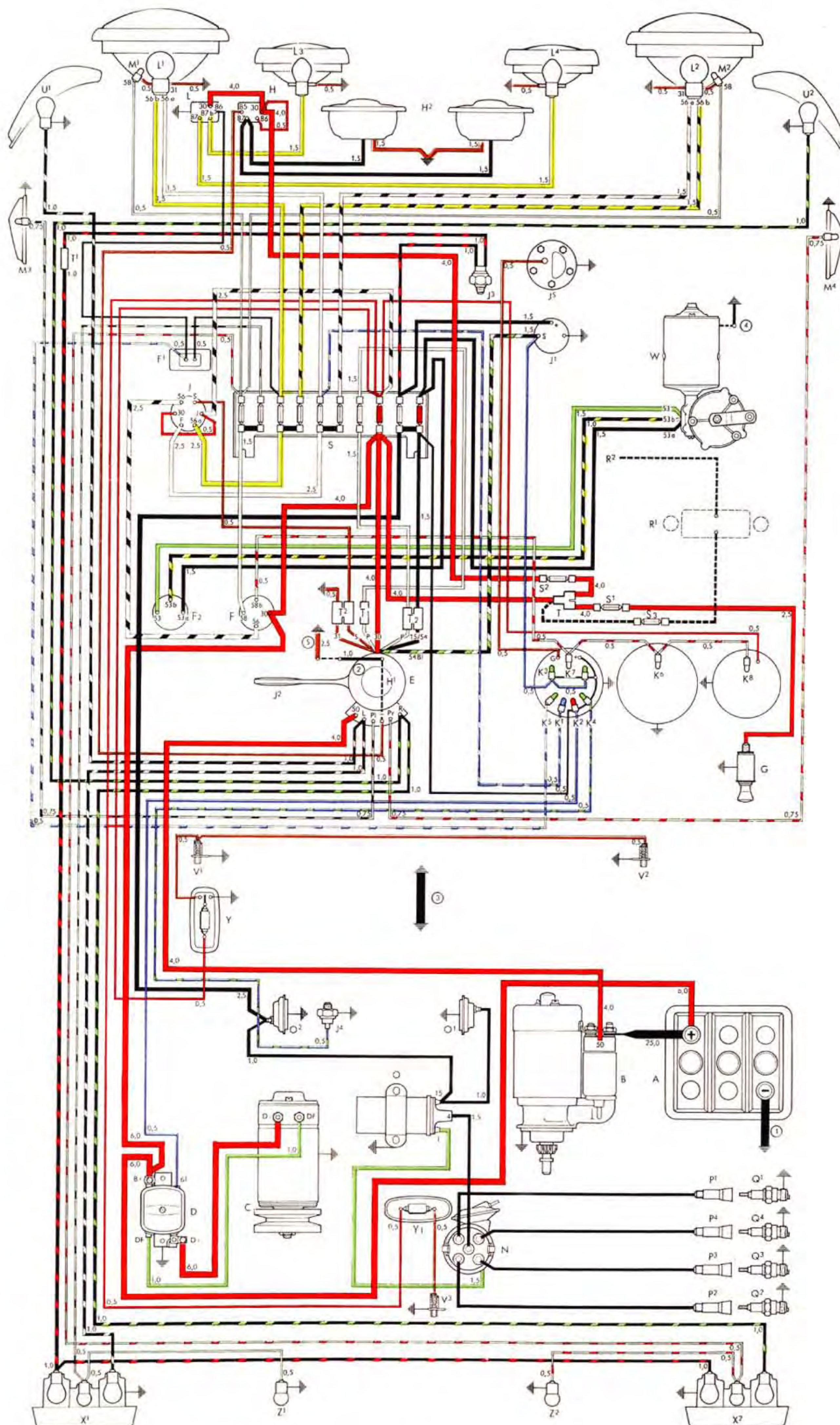
Wiring Diagram VW 1500 — Karmann Ghia Models (from May 1964, Chassis No. 0 425 853)
