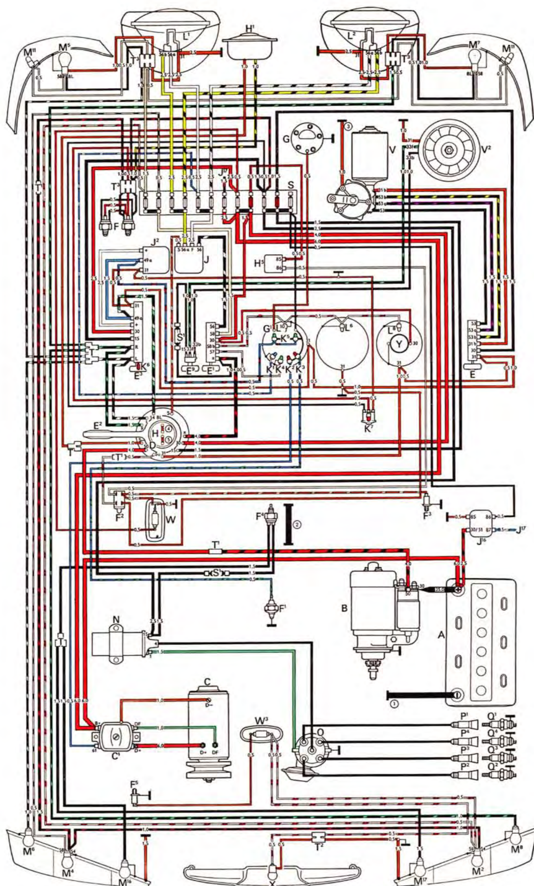
Wiring diagram VW Type 3 – from August 1970
