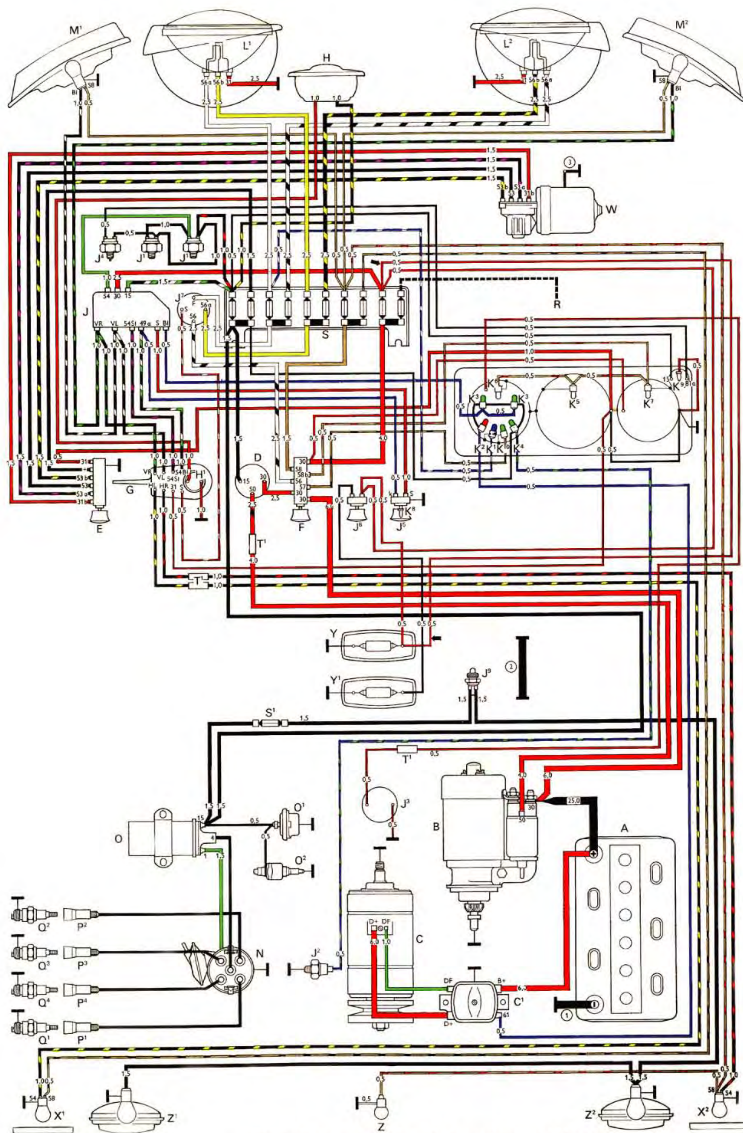
Wiring diagram VW Type 2, from August 1967 (US version)
