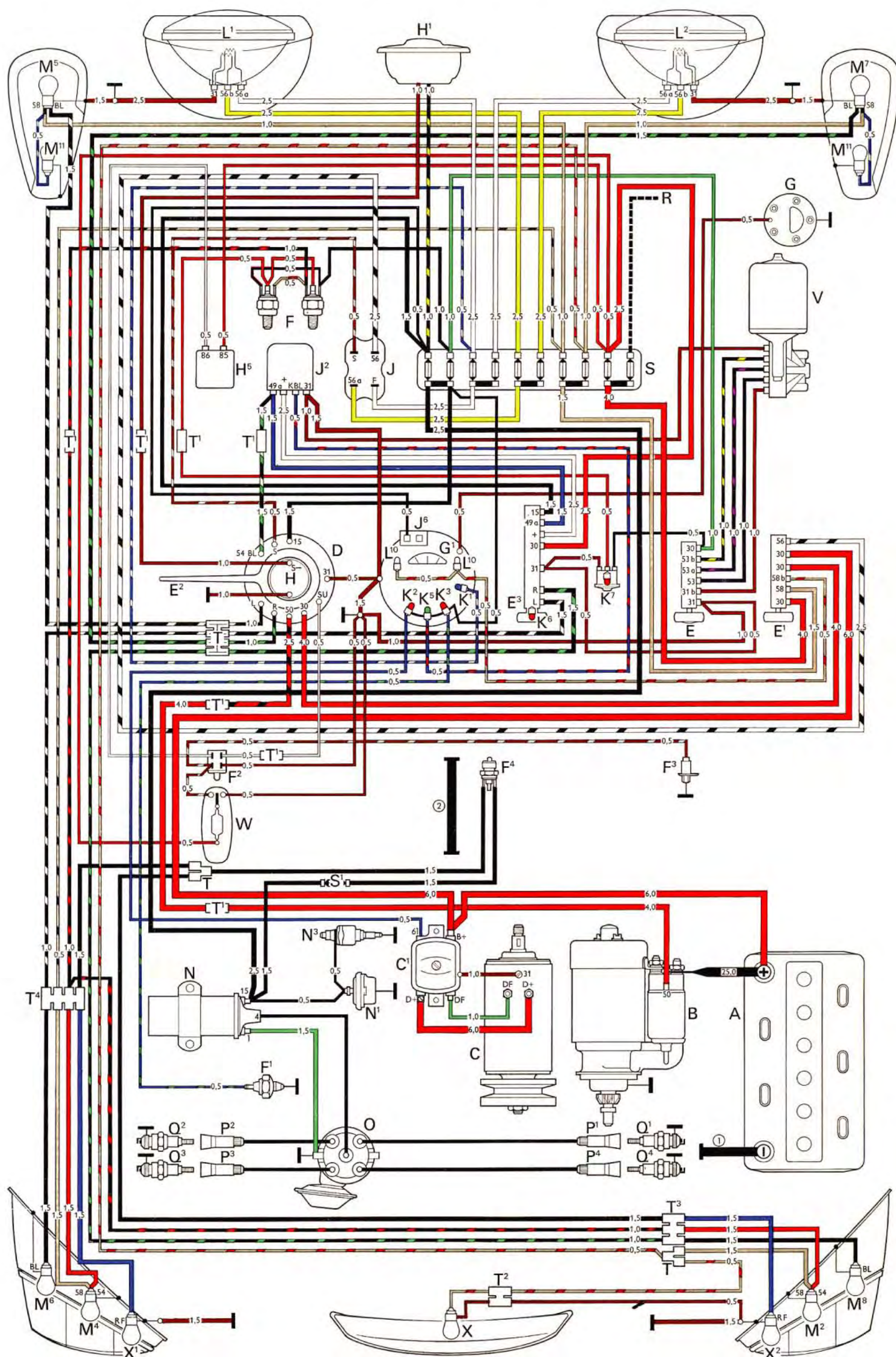
Wiring diagram VW Type 1 – from August 1969
