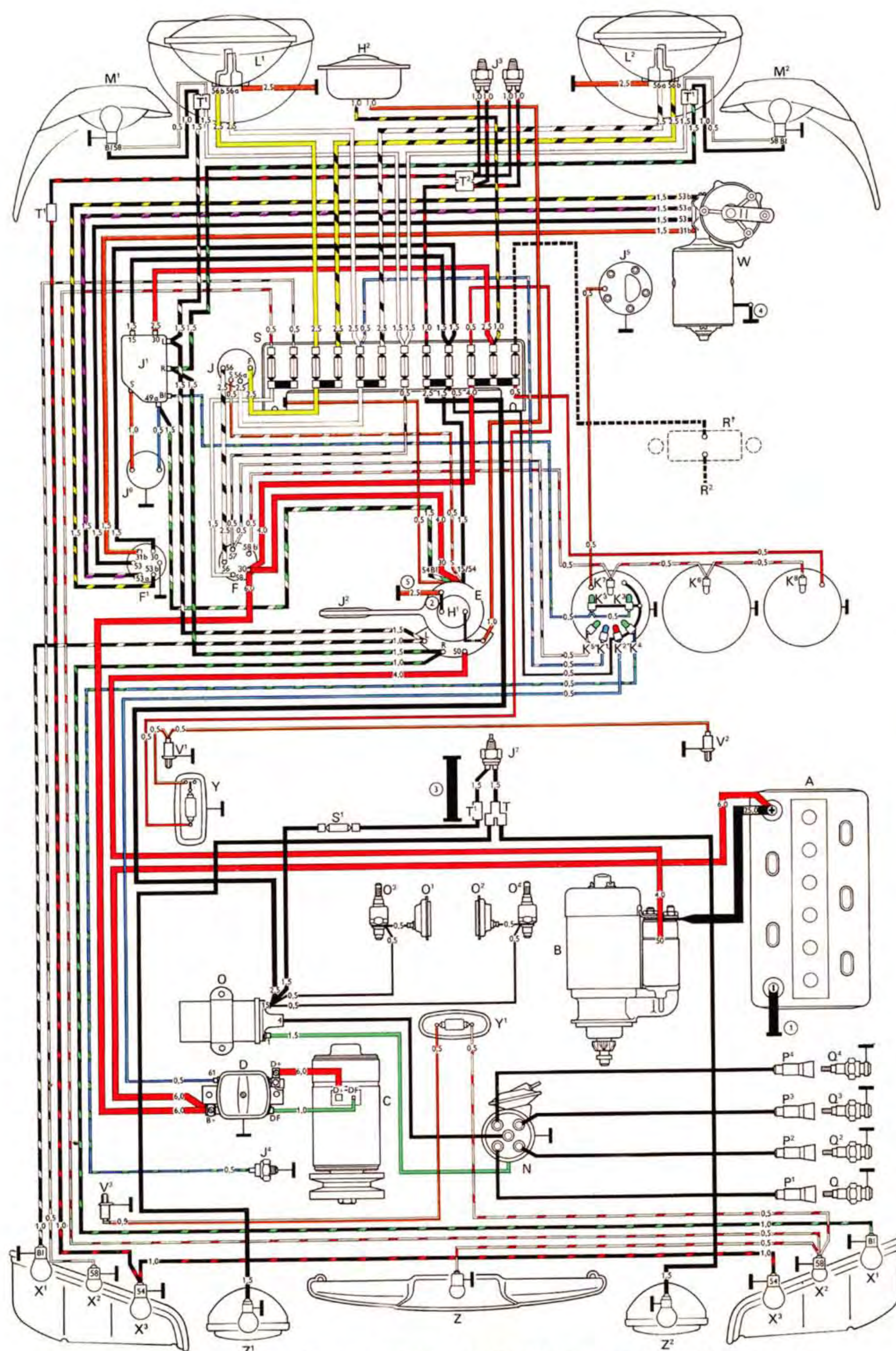
Wiring diagram VW Type 3, 1600, from August 1966 (US version)
