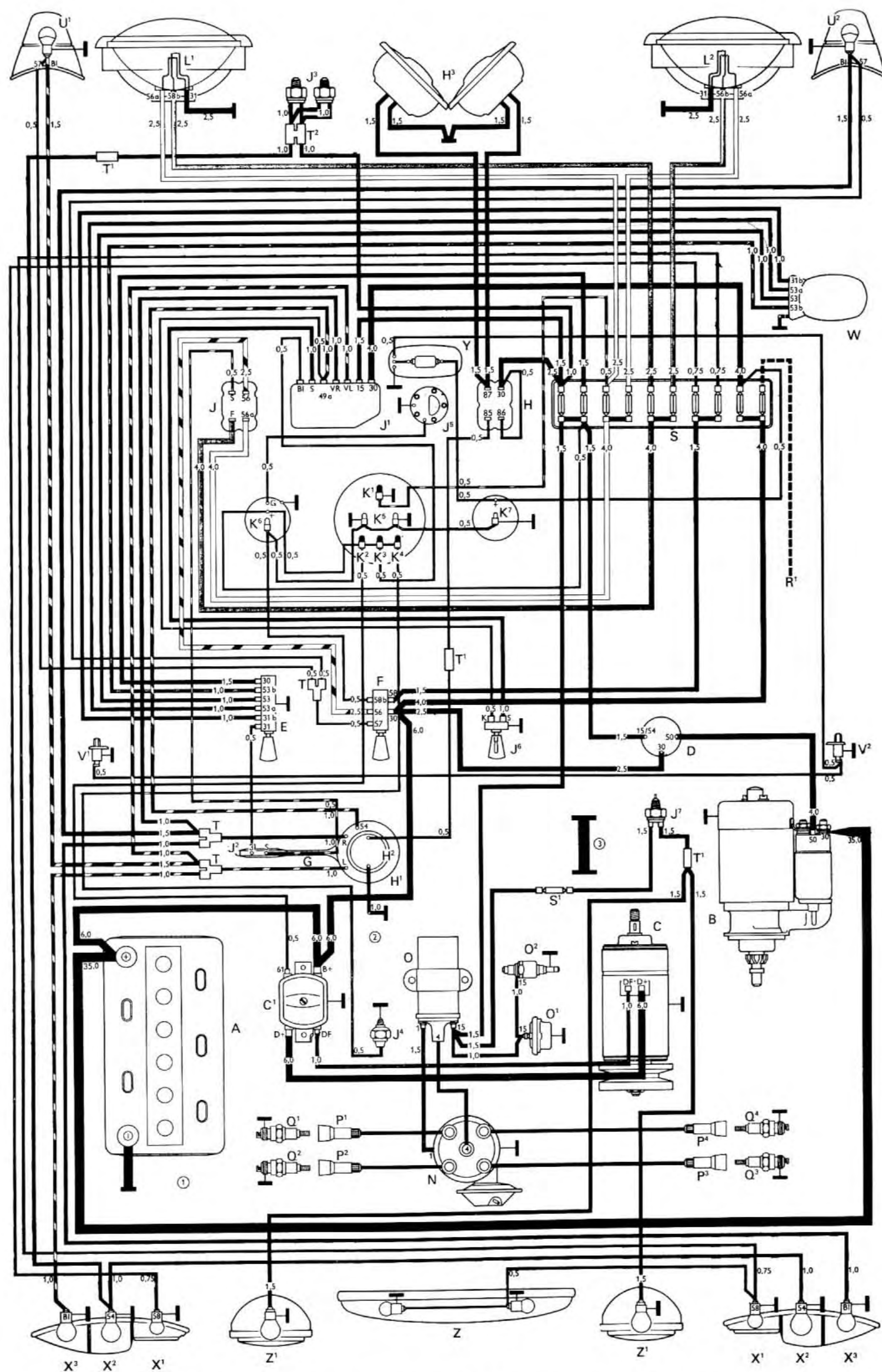
Wiring diagram VW 1500 Karmann Ghia, US version, from August 1966
