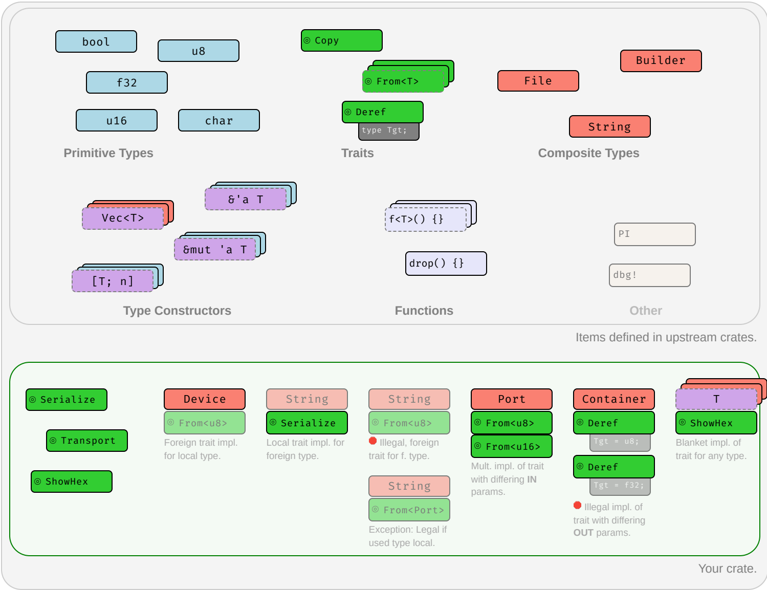
Examples of traits and types, and which traits you can implement for which type.
