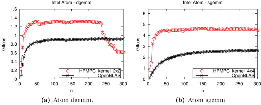
Figure 5.1: Performance test of different implementations of gemm for squared matrices of size n \times n , n \in [4, 300] , on an Intel Atom N270, code compiled with gcc 4.6.3. Peak performance in double (single) precision is 1 \cdot 1.6 = 1.6 Gflops ( 4 \cdot 1.6 = 6.4 Gflops).
