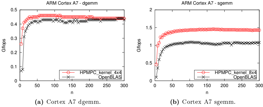
Figure 5.7: Performance test of gemm kernel for squared matrices of size n \times n , n \in [4, 300] , on an ARM Cortex A7, code compiled with gcc 4.?. Peak performance in double (single) precision is 0.5 \cdot 1 = 0.5 Gflops ( 2 \cdot 1 = 2 Gflops).
