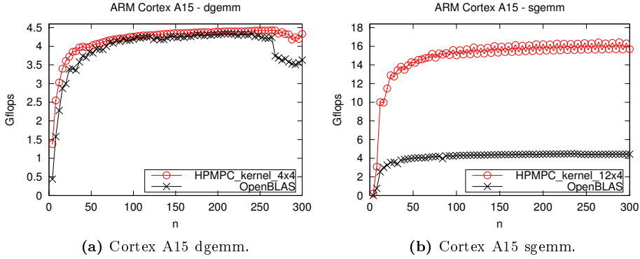
Figure 5.6: Performance test of gemm kernel for squared matrices of size n \times n , n \in [4, 300] , on an ARM Cortex A15, code compiled with gcc 4.?. Peak performance in double (single) precision is 2 \cdot 2.3 = 4.6 Gflops ( 8 \cdot 2.3 = 18.4 Gflops).
