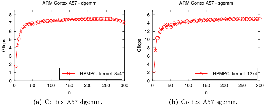
Figure 5.8: Performance test of gemm kernel for squared matrices of size n \times n , n \in [4, 300] , on an ARM Cortex A57, code compiled with gcc 4.?. Peak performance in double (single) precision is 4 \cdot 2.15 = 8.6 Gflops ( 8 \cdot 2.15 = 17.2 Gflops).
