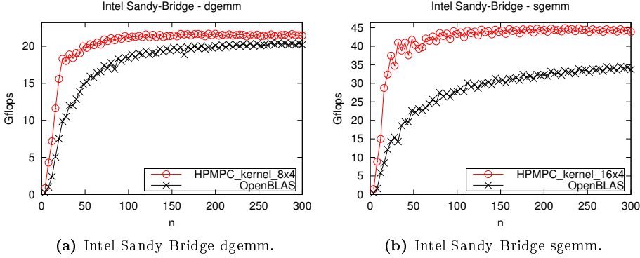
Figure 5.3: Performance test of gemm kernel for squared matrices of size n \times n , n \in [4, 300] , on an Intel Sandy-Bridge, code compiled with gcc 4.8.4. Peak performance in double (single) precision is 8 \cdot 2.9 = 23.2 Gflops ( 16 \cdot 2.9 = 46.4 Gflops).
