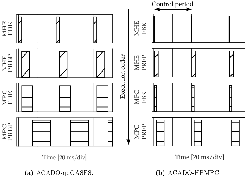
Figure 14.1: Feedback and preparation step times for the MHE and MPC using the ACADO-qpOASQS and ACADO-HPMPC solvers in the rotational start-up of an airborne wind energy system.
