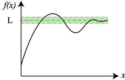
Figure 10. The function f(x) oscillates up and down initially, but then it converges (settles down) close to the value L for large values of x .
