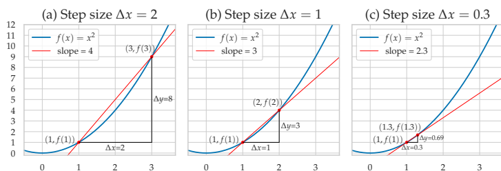
Figure 12. Calculating the slope of the line that passes through the points (x, f(x)) and (x + \Delta x, f(x + \Delta x)) for three values of the step size \Delta x .
