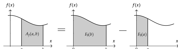
Figure 20. The area under f(x) between x = a and x = b is computed using the formula A_f(a, b) = F_0(b) - F_0(a) , which describes the change in the integral function F_0 between x = a and x = b .
