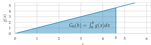
Figure 22. The integral function of the function g(x) = x is G_0(b) = \frac{1}{2}b^2 .
