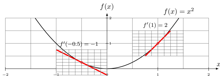
Figure 13. The derivative of the function at x = a is denoted f'(a) and describes the slope of the function at that point. You can visually confirm the slope calculation using the mini grids drawn near each point.
