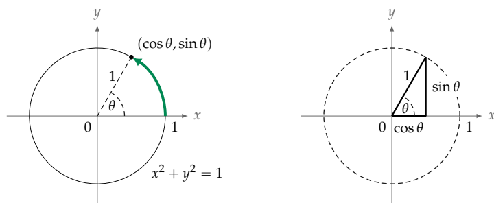
Figure 6. The coordinates of the point on the unit circle are x = \cos \theta and y = \sin \theta , where \theta is the angle the point makes with the x -axis.
