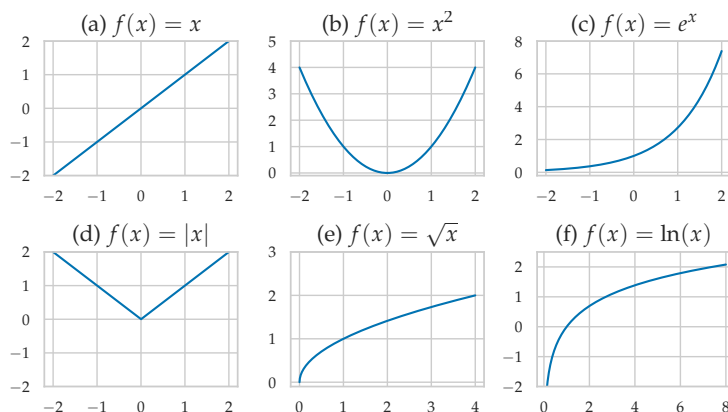
Figure 4. Graphs of six math functions that you should know about.
