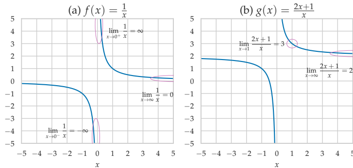
Figure 11. Visual representation of the limit calculations from the examples.
