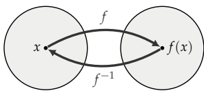
Figure 3. The inverse f^{-1} undoes the action of the function f .
