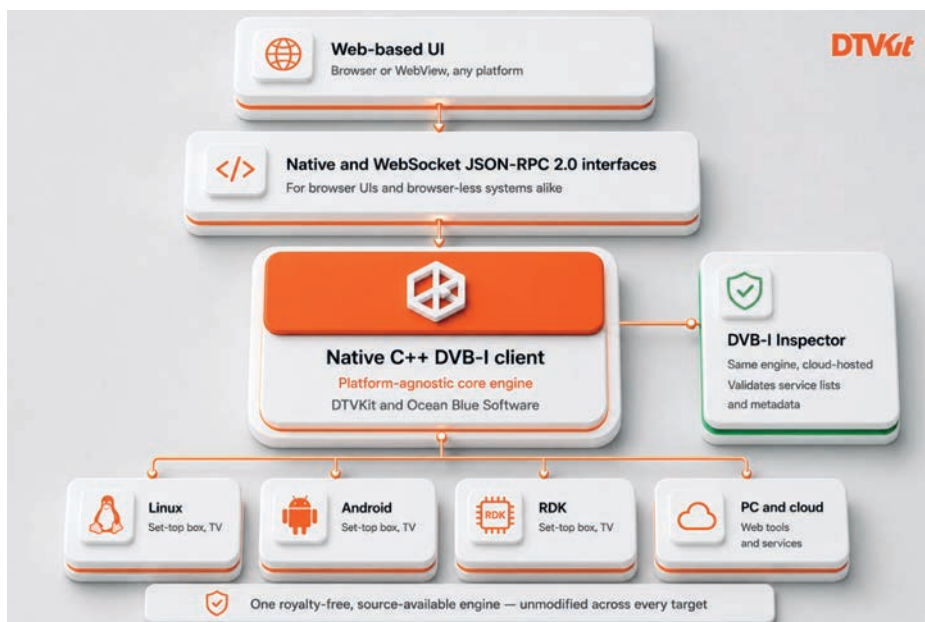
DTVKit's DVB-I architecture: one native C++ DVB-I engine, shared unmodified across Linux, Android, RDK and cloud
