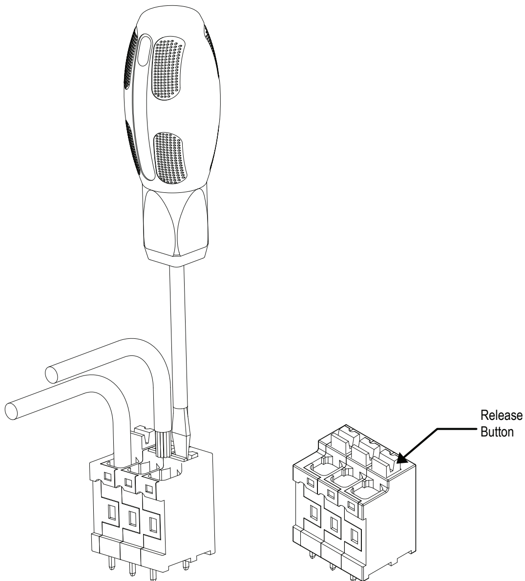
Figure 13: OMNIMATE Connector Instructions
