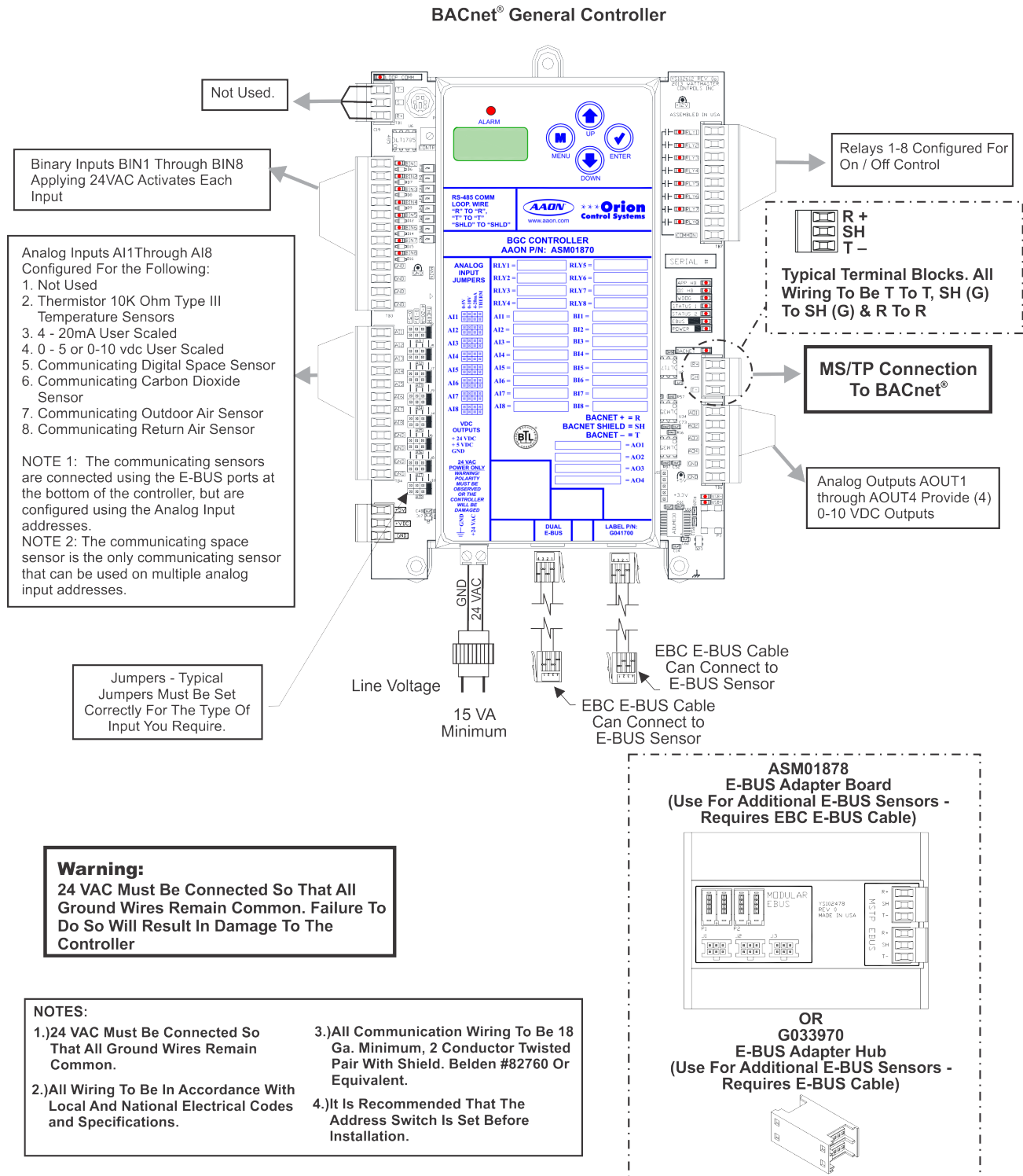
Figure 2: BGC Wiring Diagram
