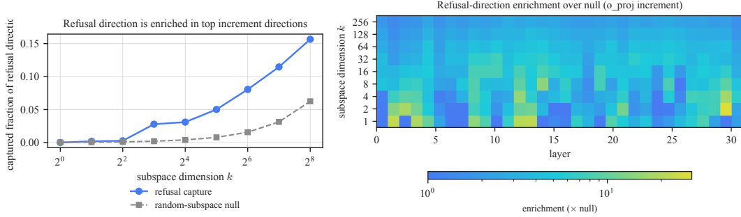
Figure 9: Left : captured fraction of the post-block-14 refusal direction by the top- k block-14 o\_proj increment subspace and the random reference. Rightward includes more directions; upward means more capture. Right : columns vary source block, rows vary k , and color gives enrichment over random.
