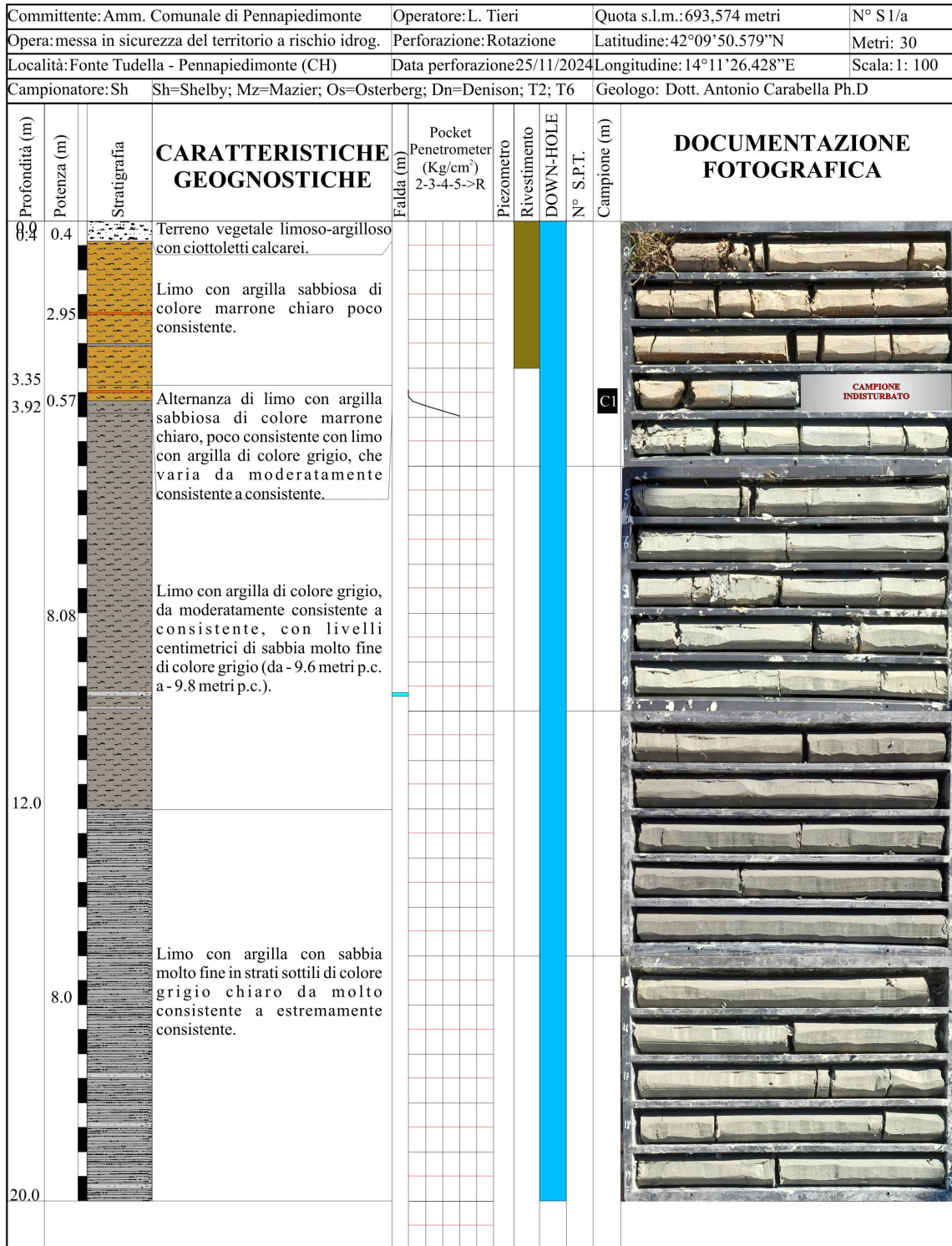
Fig. 34 : geotechnical core stratigraphy for S1 downhole VSP seismic survey. Included with permission given by Dr. Carabella.
