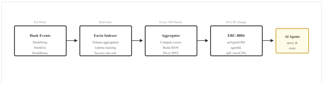
Figure 9. Dynamic metadata pipeline. Hook events are indexed in real-time by Envio, aggregated off-chain into performance scores, pinned to IPFS, and written to the ERC-8004 Identity Registry via setAgentURI . AI agents consume updated metadata to inform routing decisions.
