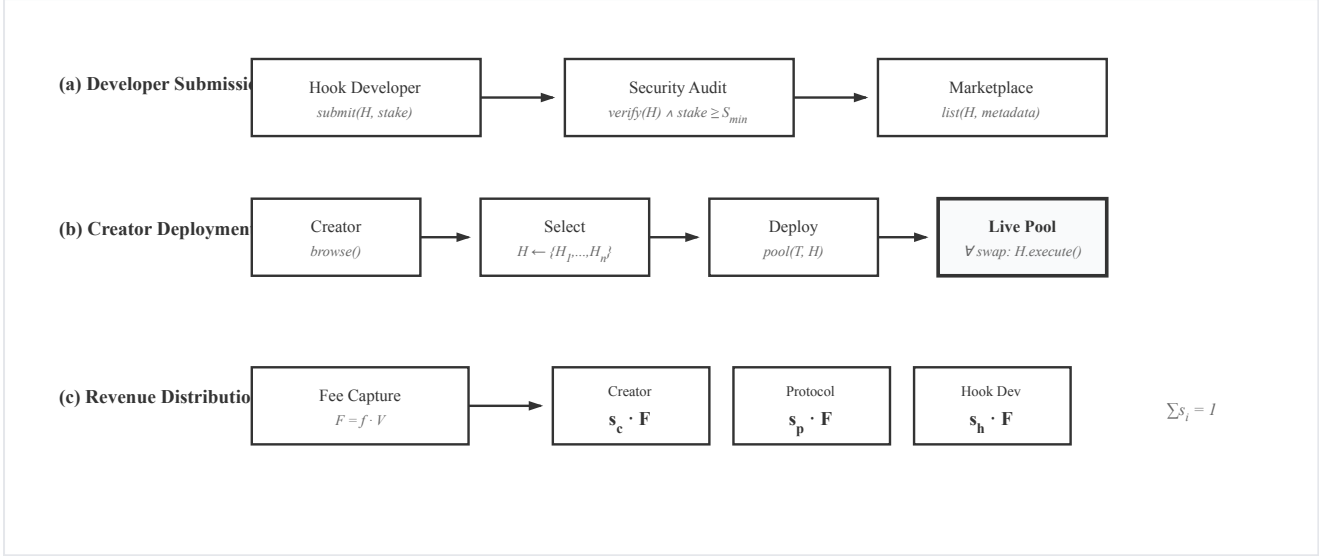
Figure 5. Hook Marketplace workflow. (a) Developers submit hooks with stake collateral; security audit verifies correctness. (b) Creators select hook set H and deploy pool. (c) Swap fees F distributed according to share vector (s_c, s_p, s_h) where s_c + s_p + s_h = 1 .
