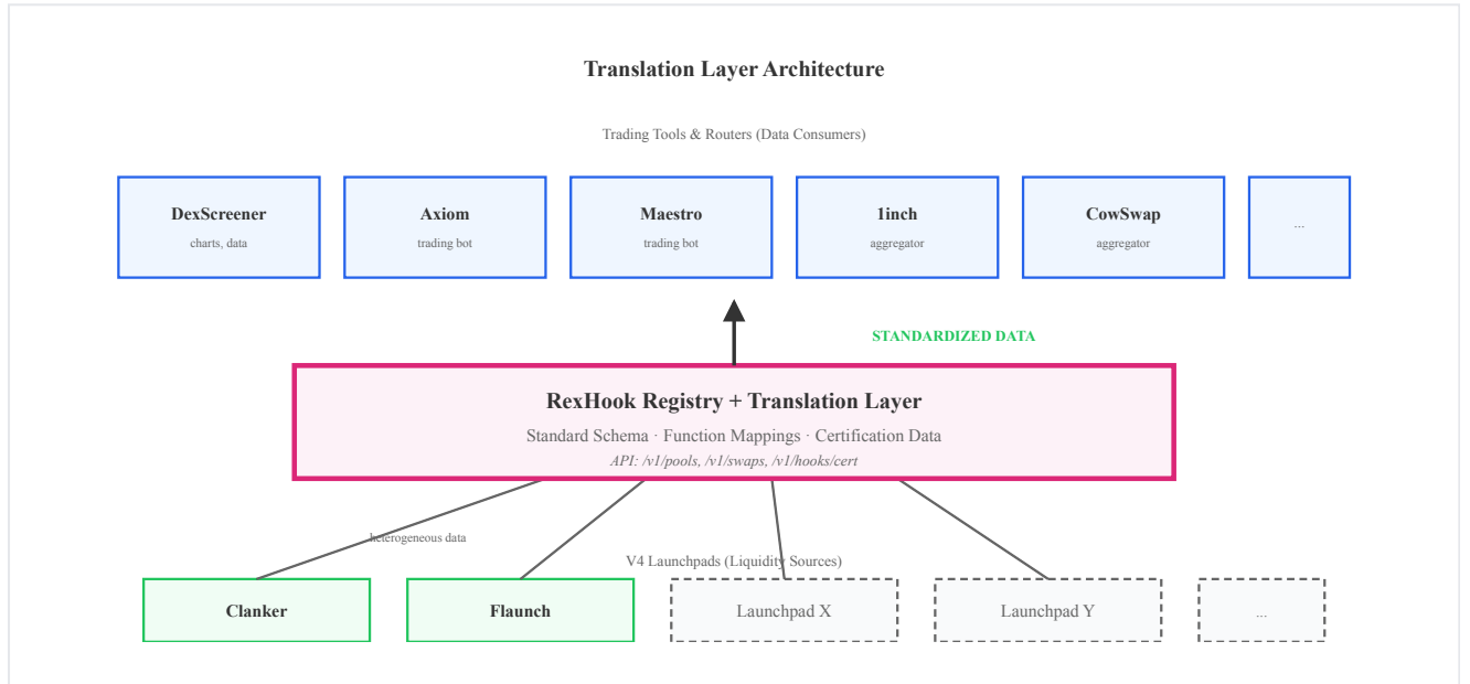
Figure 7b. Translation layer architecture. V4 launchpads (Clanker, Flaunch, etc.) provide liquidity with heterogeneous interfaces. RexHook Registry standardizes this data. Trading tools and routers consume standardized data via a single integration—they don't need custom adapters for each launchpad.
