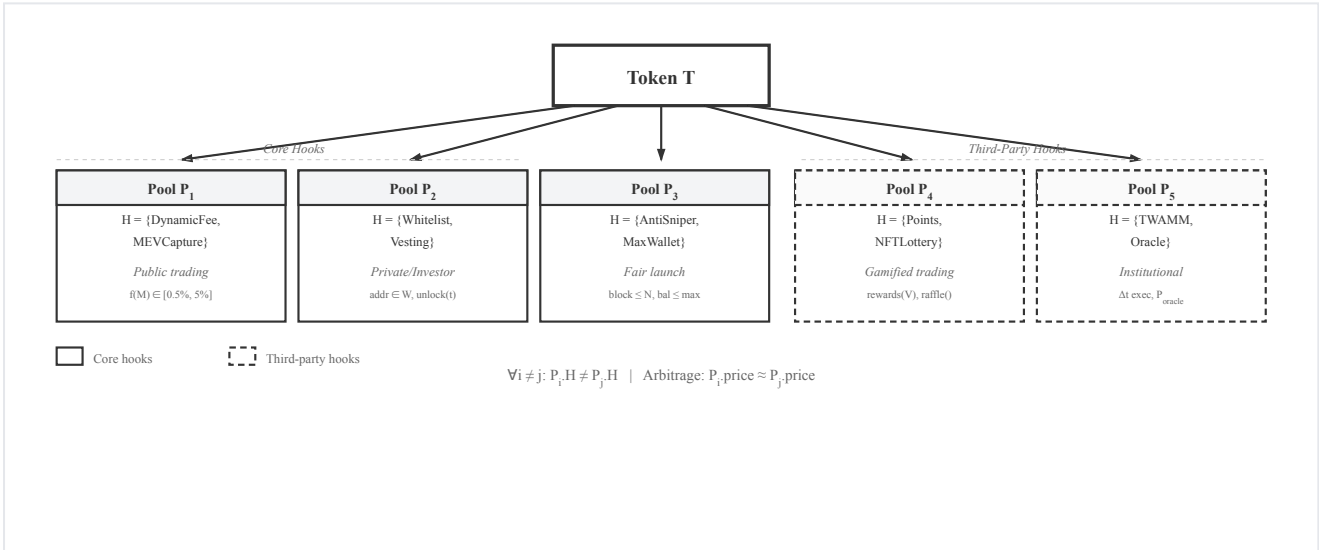
Figure 6. Multi-pool architecture for token T . Each pool P_i binds a distinct hook set H_i . Core hooks (solid border): P_1 public trading, P_2 private investors, P_3 fair launch protection. Third-party hooks (dashed border): P_4 gamified rewards, P_5 institutional TWAMM with oracle pricing. Arbitrage between pools maintains price consistency across all configurations.
