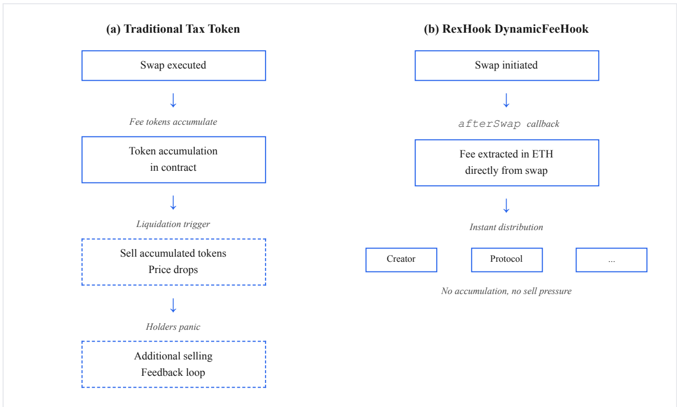
Figure 1. Comparative flow diagrams for (a) traditional tax token fee mechanics showing the feedback loop leading to death spiral, and (b) RexHook's DynamicFeeHook achieving zero additional sell pressure through in-swap ETH extraction.
