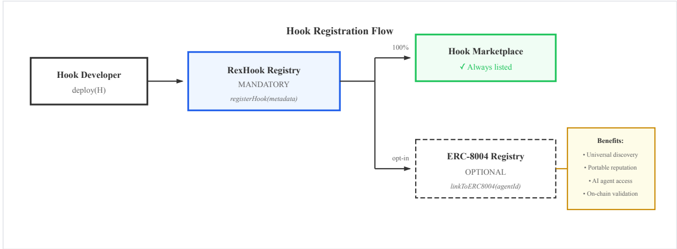
Figure 7. Hook registration flow. All hooks are registered in the RexHook Registry (mandatory). Developers can optionally link to ERC-8004 for universal discovery and portable reputation.
